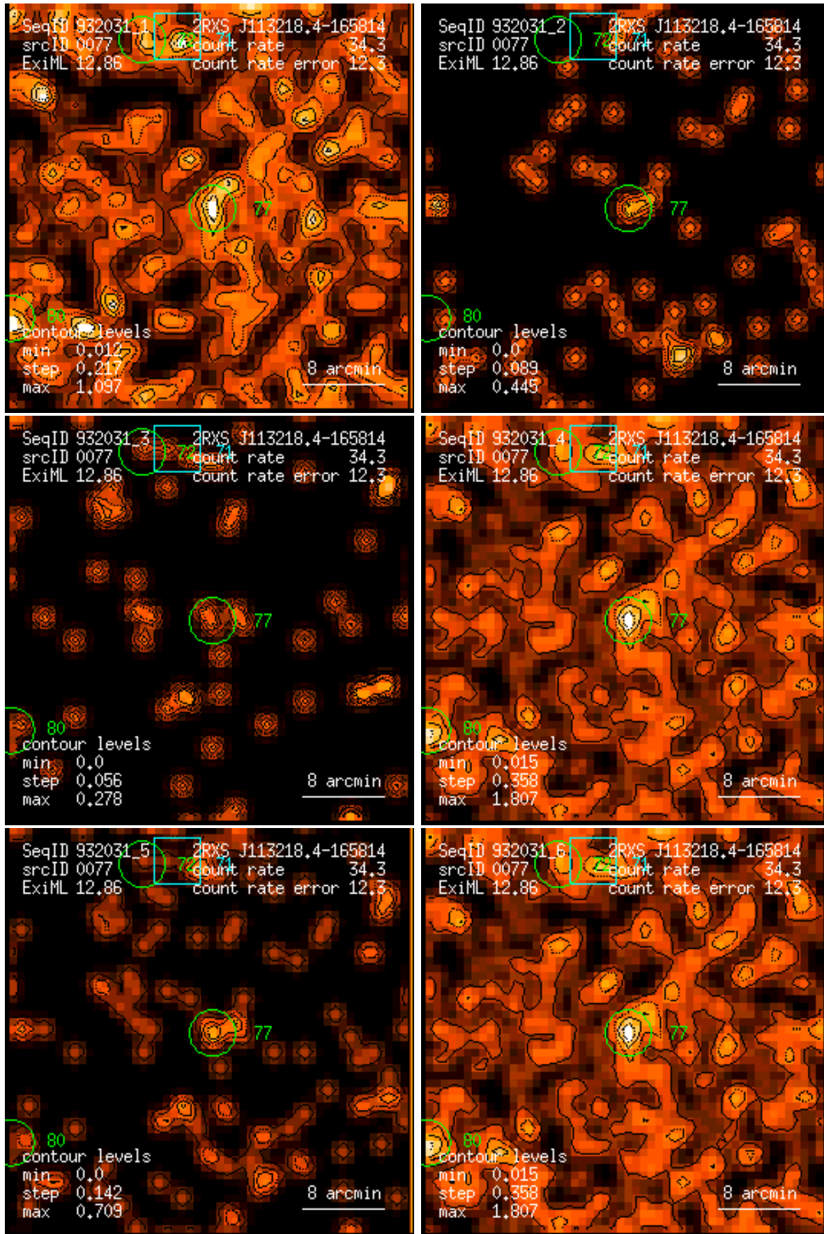
Figure 77: RASS 932031: detection 0077: band rate images, Gaussian filter: (1) PSPC channels 11 – 41, (2) 52 – 90, (3) 91 – 201, (4) 11 – 235, (5) 52 – 201, (6) 11 – 201. Broad band rates in counts/ks. Band rate contour levels in counts/ks/arcmin 2 .
