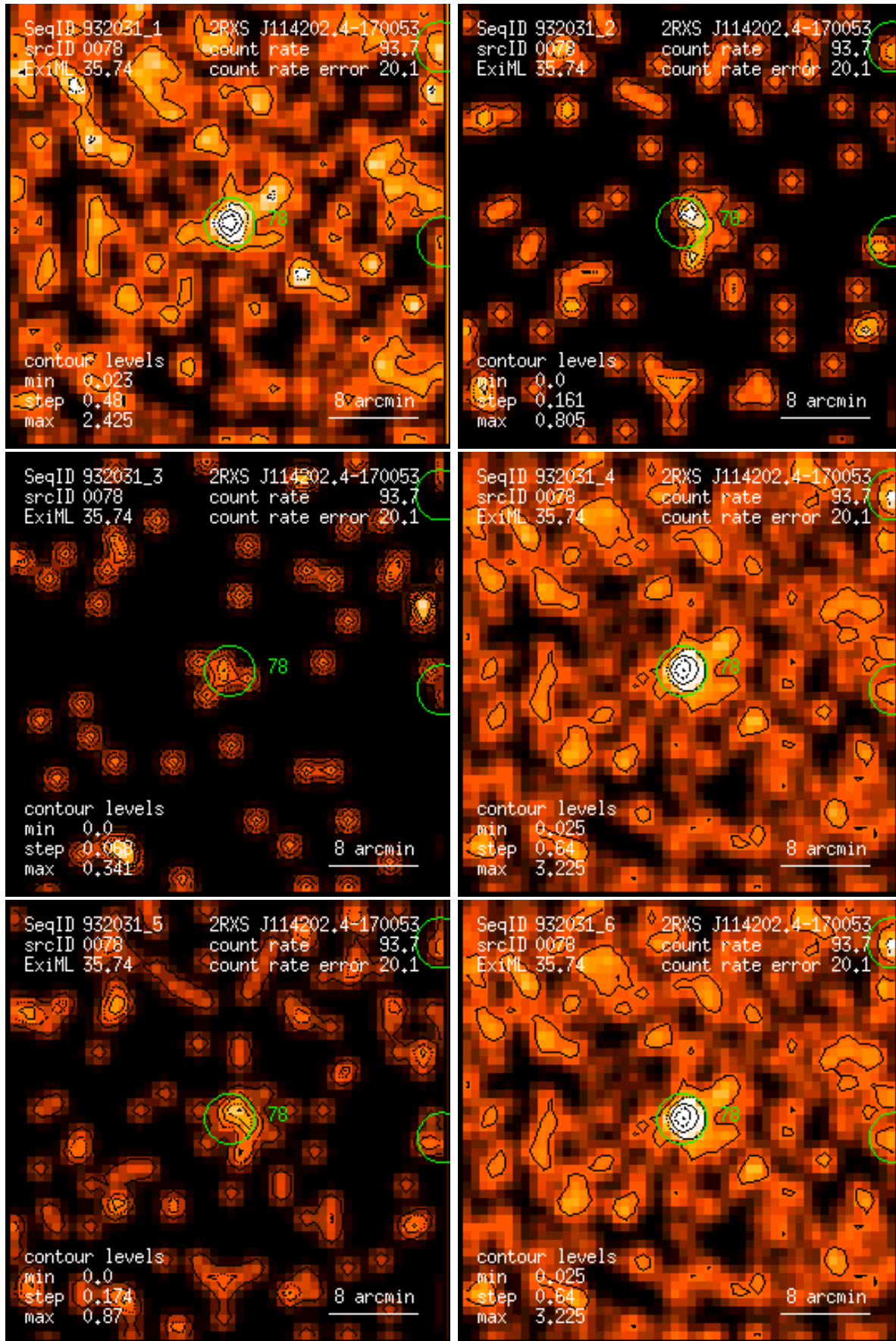
Figure 78: RASS 932031: detection 0078: band rate images, Gaussian filter: (1) PSPC channels 11 – 41, (2) 52 – 90, (3) 91 – 201, (4) 11 – 235, (5) 52 – 201, (6) 11 – 201. Broad band rates in counts/ks. Band rate contour levels in counts/ks/arcmin 2 .
