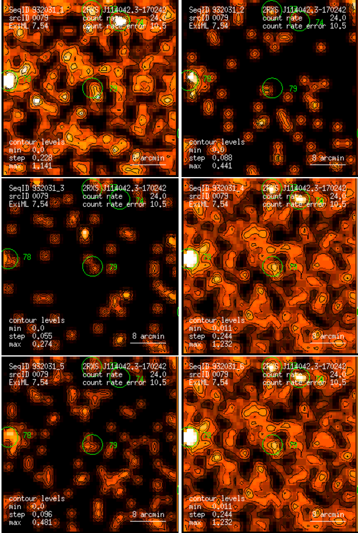
Figure 79: RASS 932031: detection 0079: band rate images, Gaussian filter: (1) PSPC channels 11 – 41, (2) 52 – 90, (3) 91 – 201, (4) 11 – 235, (5) 52 – 201, (6) 11 – 201. Broad band rates in counts/ks. Band rate contour levels in counts/ks/arcmin 2 .
