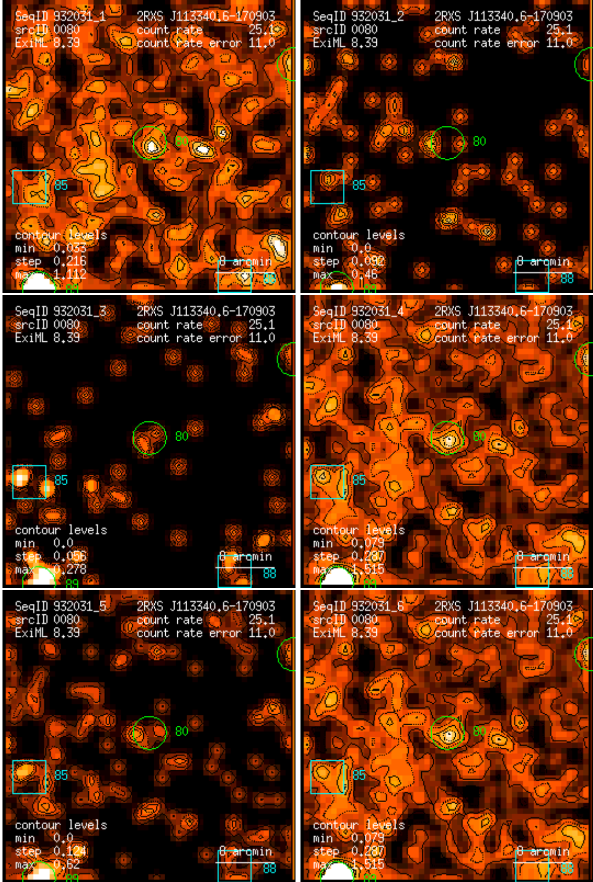
Figure 80: RASS 932031: detection 0080: band rate images, Gaussian filter: (1) PSPC channels 11 – 41, (2) 52 – 90, (3) 91 – 201, (4) 11 – 235, (5) 52 – 201, (6) 11 – 201. Broad band rates in counts/ks. Band rate contour levels in counts/ks/arcmin 2 .
