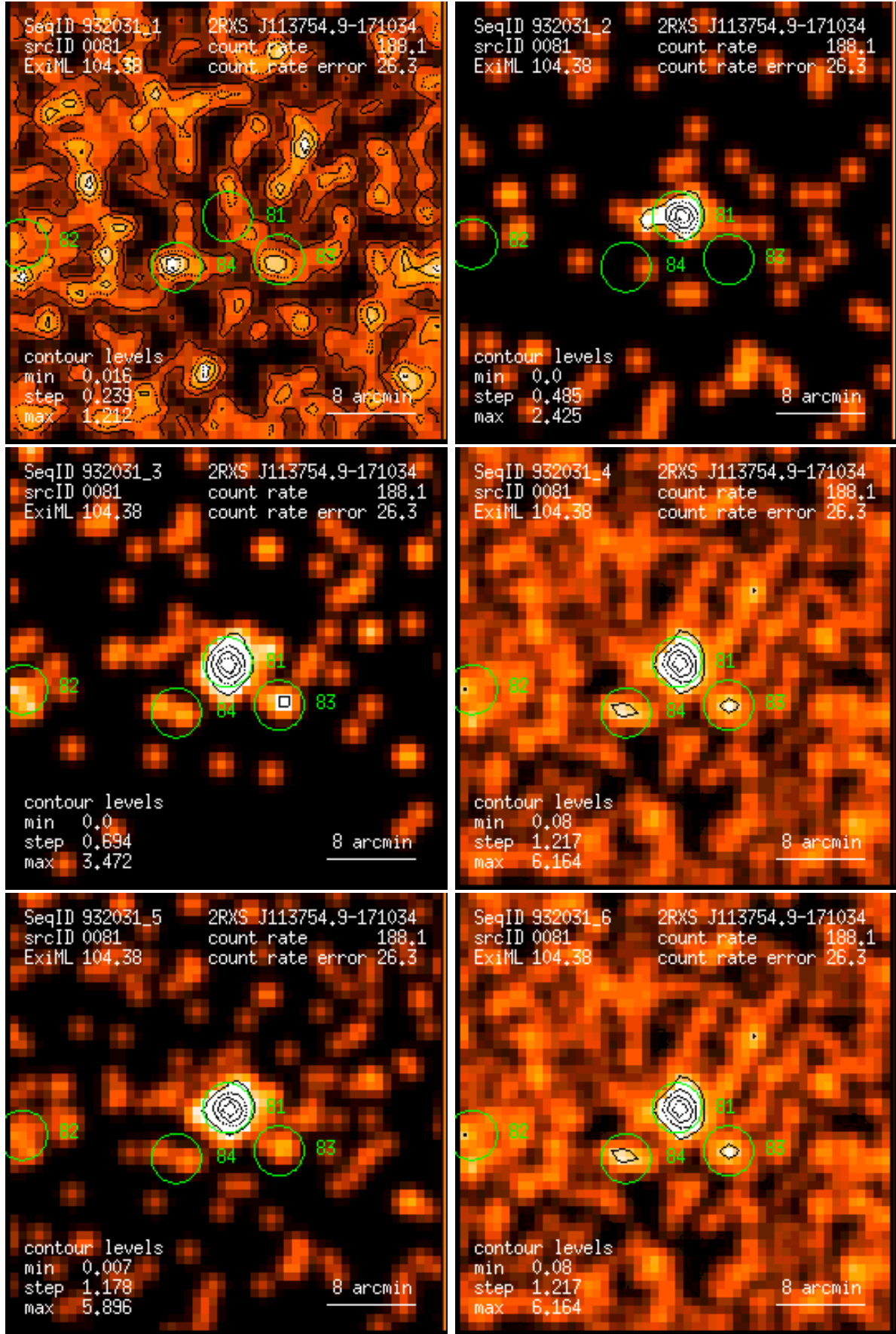
Figure 81: RASS 932031: detection 0081: band rate images, Gaussian filter: (1) PSPC channels 11 – 41, (2) 52 – 90, (3) 91 – 201, (4) 11 – 235, (5) 52 – 201, (6) 11 – 201. Broad band rates in counts/ks. Band rate contour levels in counts/ks/arcmin 2 .
