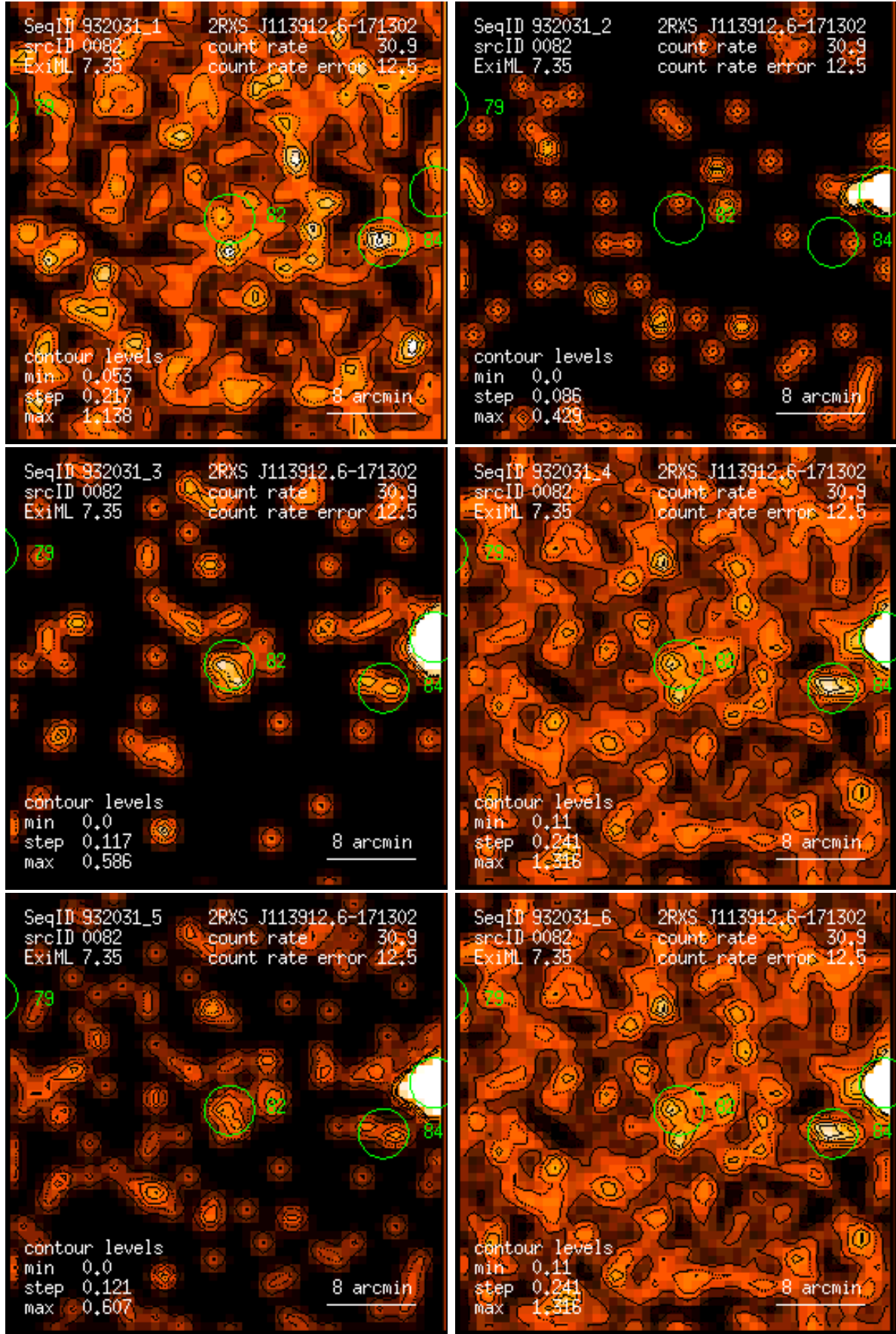
Figure 82: RASS 932031: detection 0082: band rate images, Gaussian filter: (1) PSPC channels 11 – 41, (2) 52 – 90, (3) 91 – 201, (4) 11 – 235, (5) 52 – 201, (6) 11 – 201. Broad band rates in counts/ks. Band rate contour levels in counts/ks/arcmin 2 .
