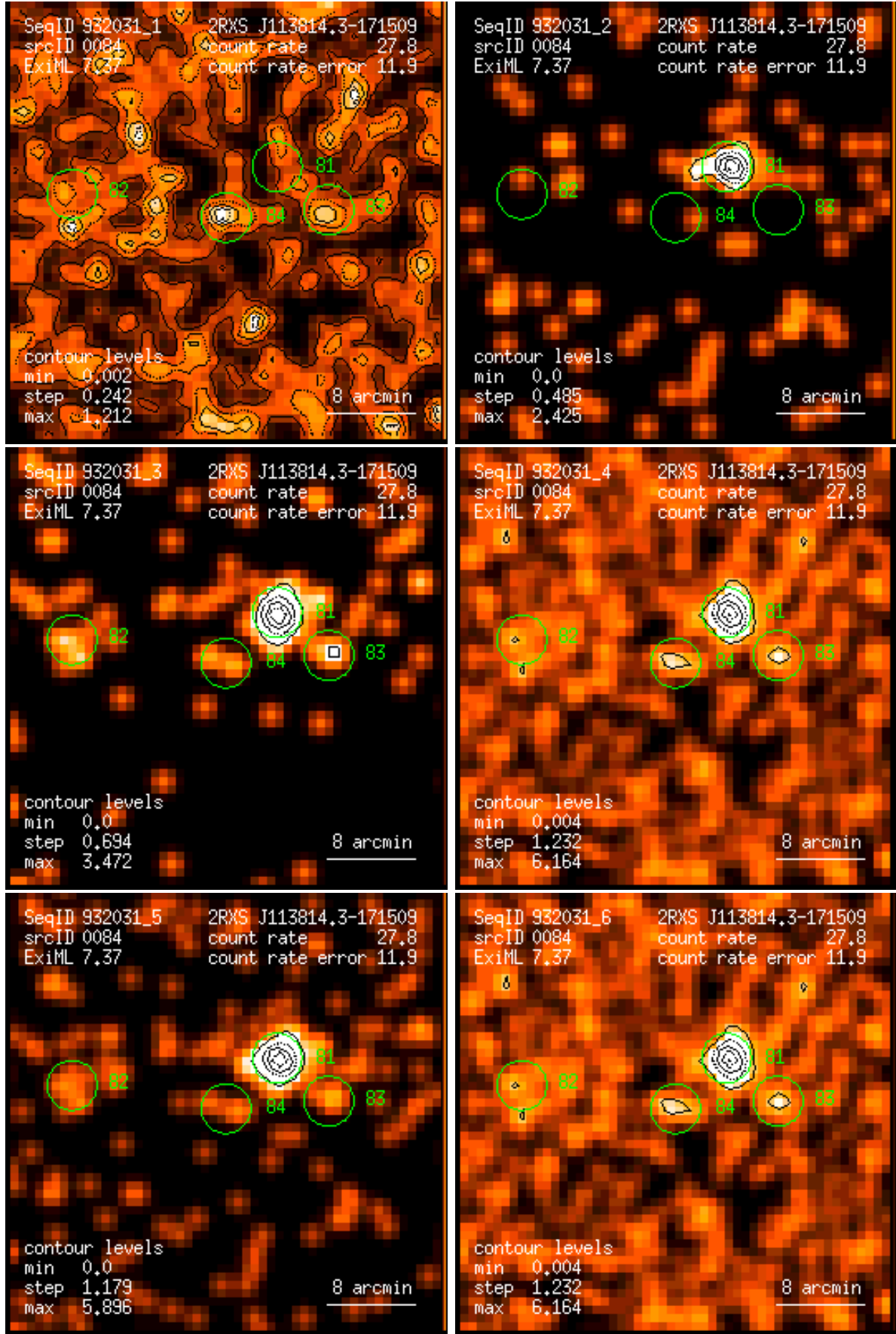
Figure 84: RASS 932031: detection 0084: band rate images, Gaussian filter: (1) PSPC channels 11 – 41, (2) 52 – 90, (3) 91 – 201, (4) 11 – 235, (5) 52 – 201, (6) 11 – 201. Broad band rates in counts/ks. Band rate contour levels in counts/ks/arcmin 2 .
