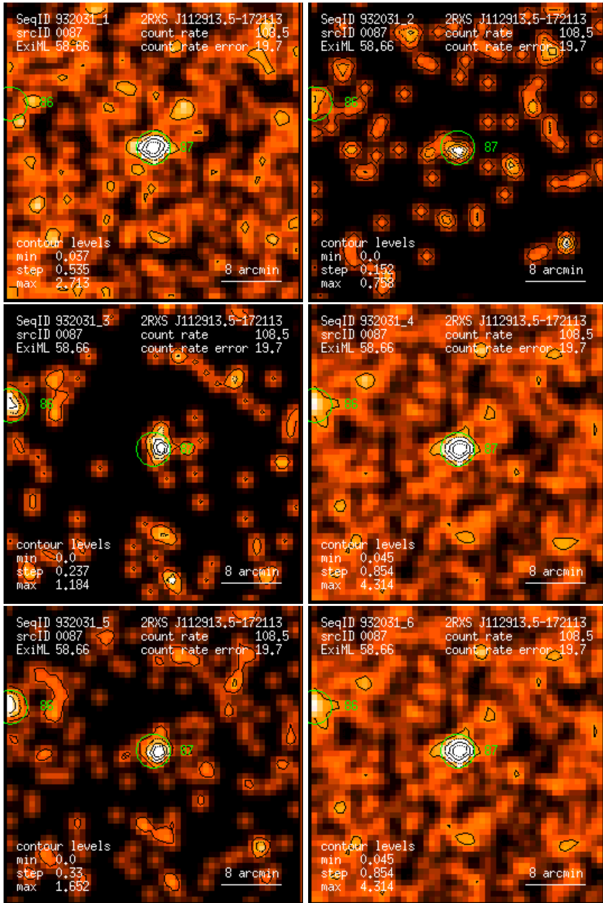
Figure 87: RASS 932031: detection 0087: band rate images, Gaussian filter: (1) PSPC channels 11 – 41, (2) 52 – 90, (3) 91 – 201, (4) 11 – 235, (5) 52 – 201, (6) 11 – 201. Broad band rates in counts/ks. Band rate contour levels in counts/ks/arcmin 2 .
