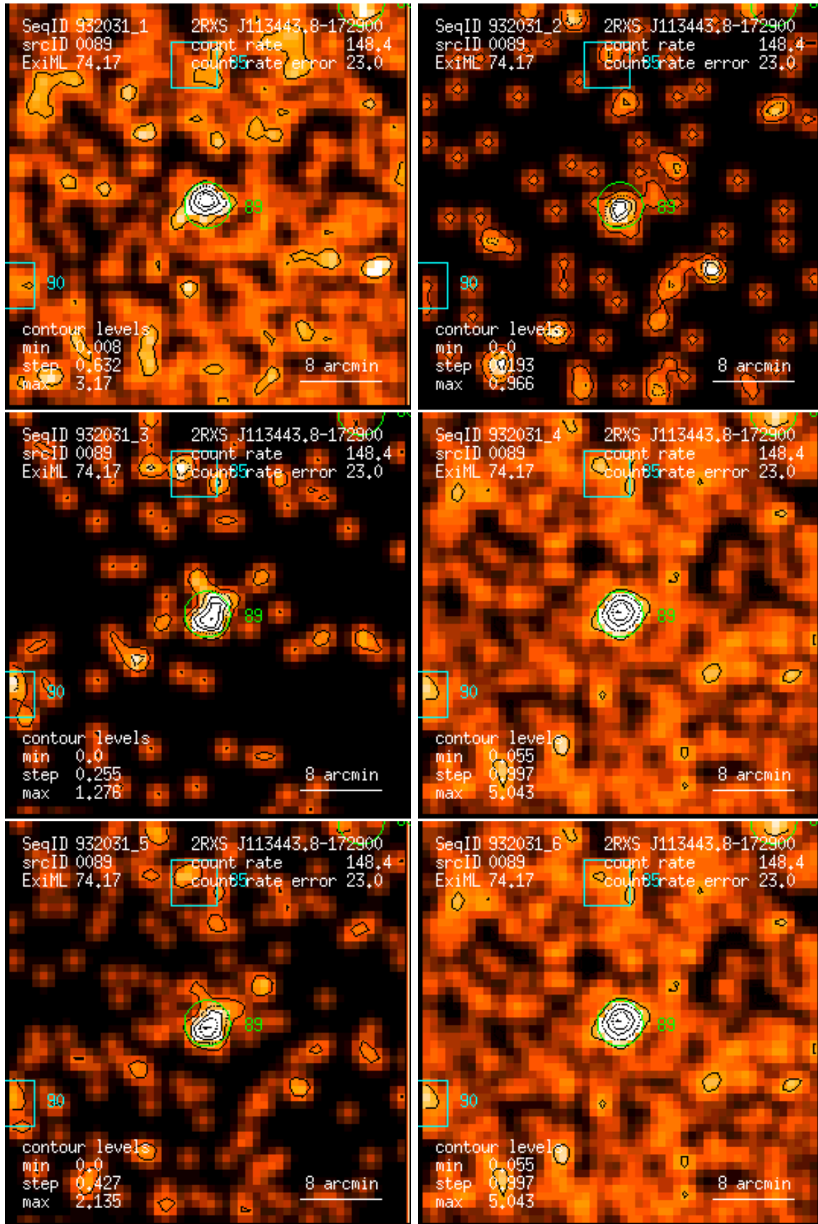
Figure 89: RASS 932031: detection 0089: band rate images, Gaussian filter: (1) PSPC channels 11 – 41, (2) 52 – 90, (3) 91 – 201, (4) 11 – 235, (5) 52 – 201, (6) 11 – 201. Broad band rates in counts/ks. Band rate contour levels in counts/ks/arcmin 2 .
