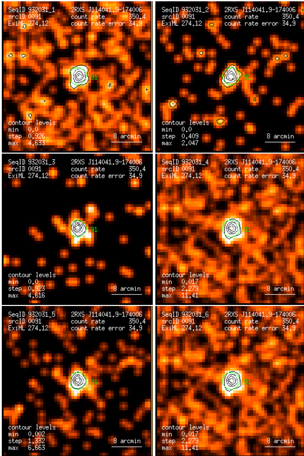
Figure 91: RASS 932031: detection 0091: band rate images, Gaussian filter: (1) PSPC channels 11 – 41, (2) 52 – 90, (3) 91 – 201, (4) 11 – 235, (5) 52 – 201, (6) 11 – 201. Broad band rates in counts/ks. Band rate contour levels in counts/ks/arcmin 2 .
