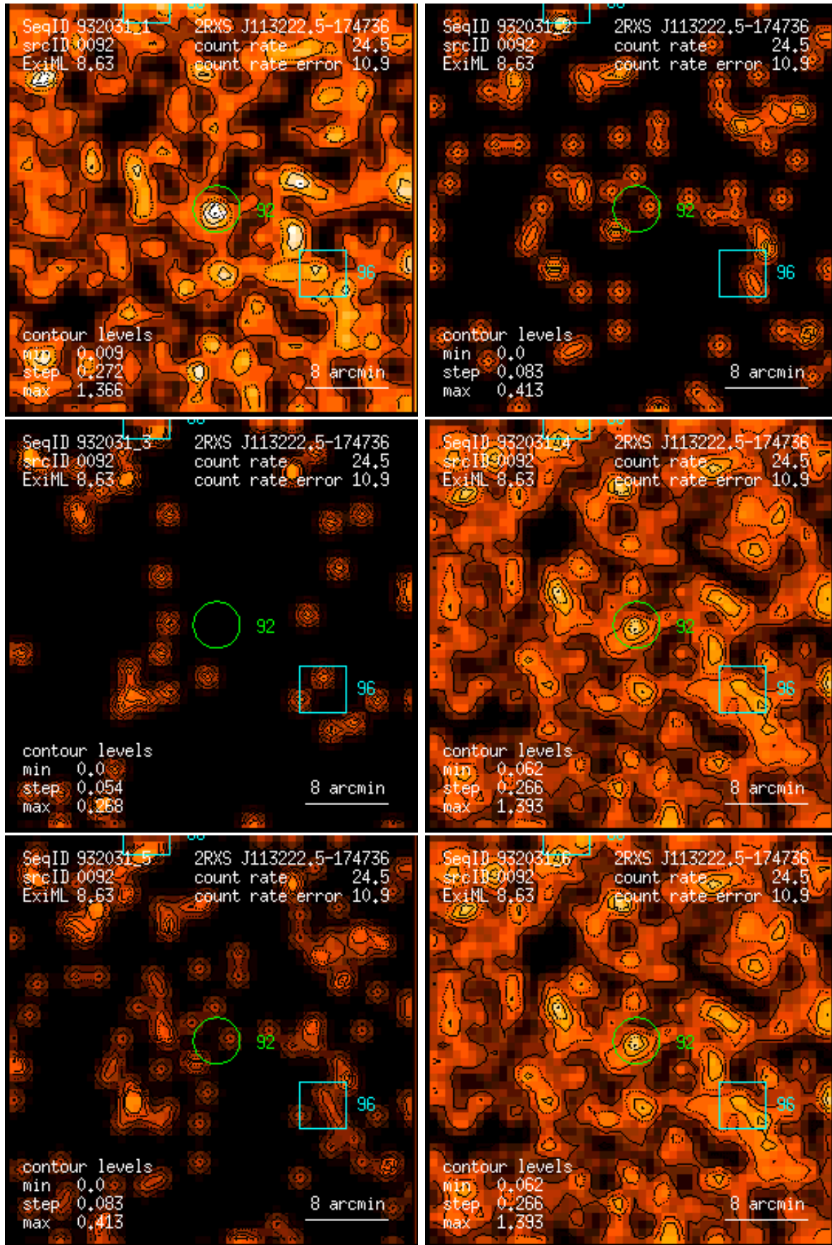
Figure 92: RASS 932031: detection 0092: band rate images, Gaussian filter: (1) PSPC channels 11 – 41, (2) 52 – 90, (3) 91 – 201, (4) 11 – 235, (5) 52 – 201, (6) 11 – 201. Broad band rates in counts/ks. Band rate contour levels in counts/ks/arcmin 2 .
