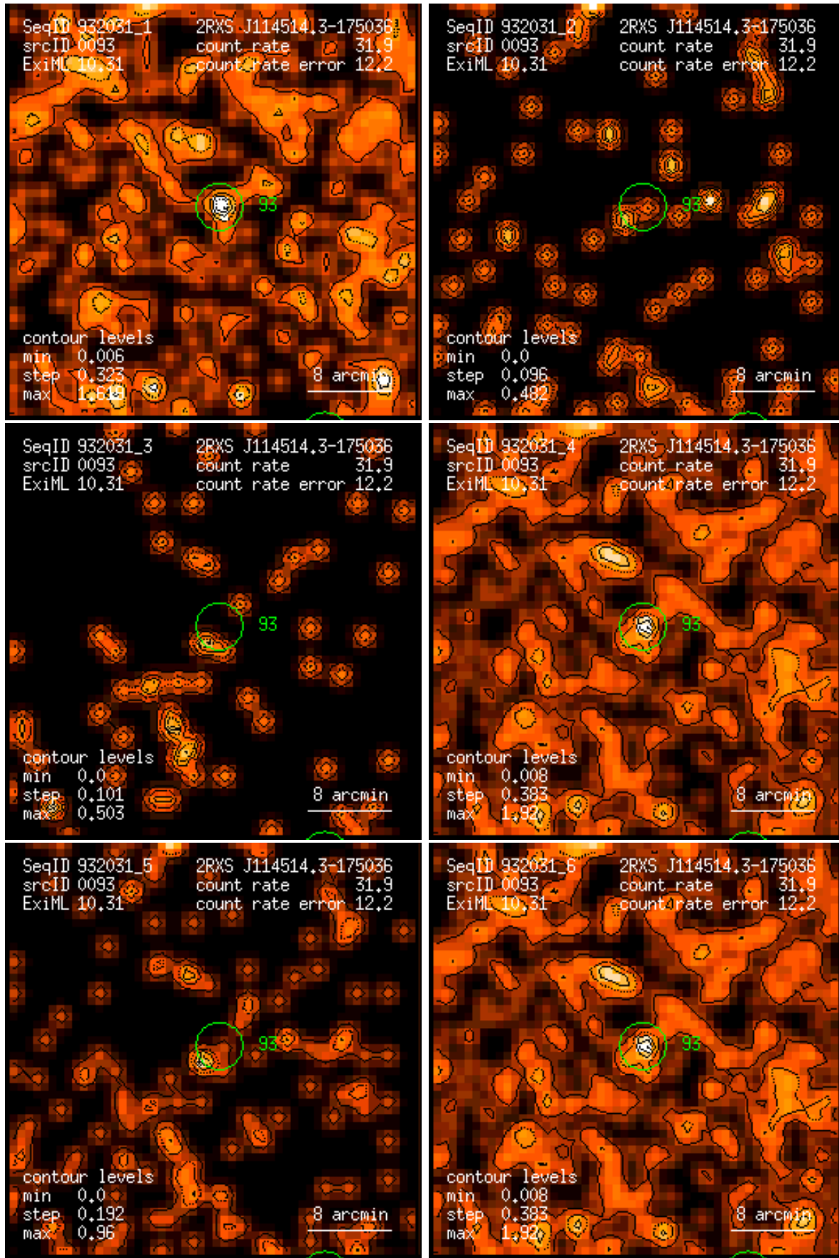
Figure 93: RASS 932031: detection 0093: band rate images, Gaussian filter: (1) PSPC channels 11 – 41, (2) 52 – 90, (3) 91 – 201, (4) 11 – 235, (5) 52 – 201, (6) 11 – 201. Broad band rates in counts/ks. Band rate contour levels in counts/ks/arcmin 2 .
