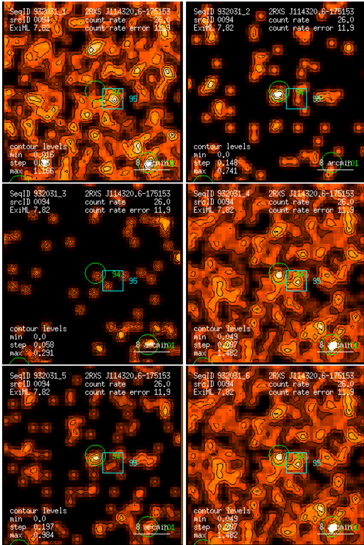
Figure 94: RASS 932031: detection 0094: band rate images, Gaussian filter: (1) PSPC channels 11 – 41, (2) 52 – 90, (3) 91 – 201, (4) 11 – 235, (5) 52 – 201, (6) 11 – 201. Broad band rates in counts/ks. Band rate contour levels in counts/ks/arcmin 2 .
