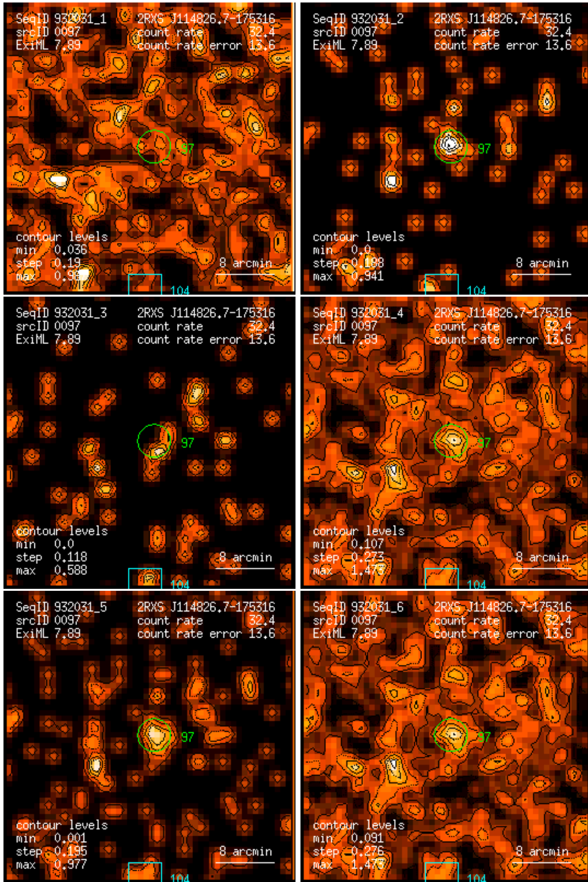
Figure 97: RASS 932031: detection 0097: band rate images, Gaussian filter: (1) PSPC channels 11 – 41, (2) 52 – 90, (3) 91 – 201, (4) 11 – 235, (5) 52 – 201, (6) 11 – 201. Broad band rates in counts/ks. Band rate contour levels in counts/ks/arcmin 2 .
