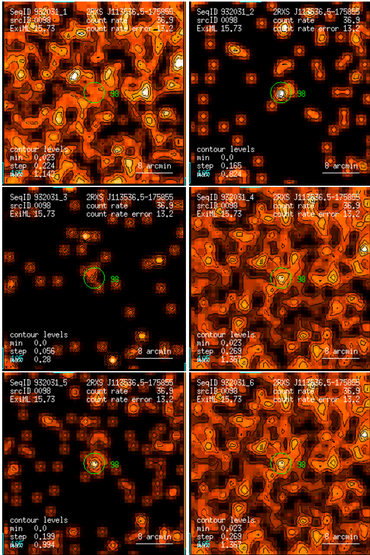
Figure 98: RASS 932031: detection 0098: band rate images, Gaussian filter: (1) PSPC channels 11 – 41, (2) 52 – 90, (3) 91 – 201, (4) 11 – 235, (5) 52 – 201, (6) 11 – 201. Broad band rates in counts/ks. Band rate contour levels in counts/ks/arcmin 2 .
