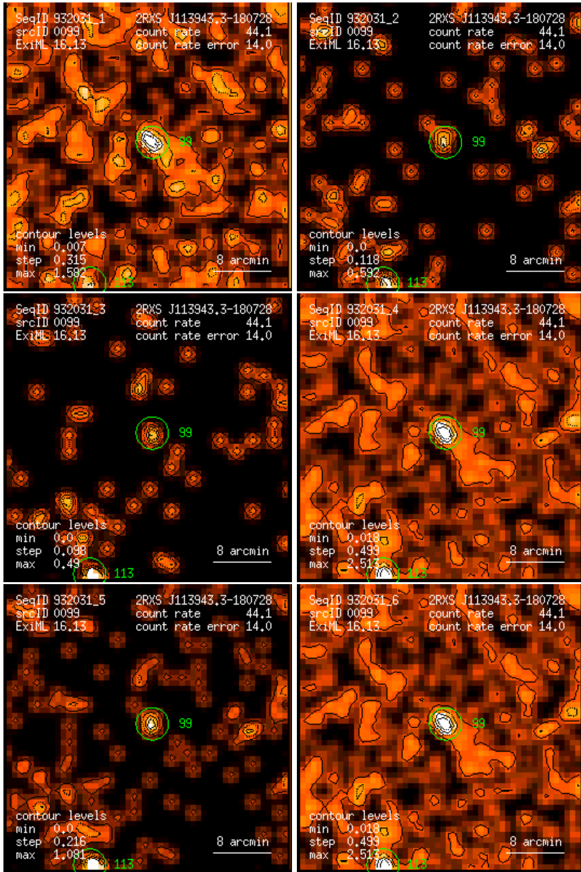
Figure 99: RASS 932031: detection 0099: band rate images, Gaussian filter: (1) PSPC channels 11 – 41, (2) 52 – 90, (3) 91 – 201, (4) 11 – 235, (5) 52 – 201, (6) 11 – 201. Broad band rates in counts/ks. Band rate contour levels in counts/ks/arcmin 2 .
