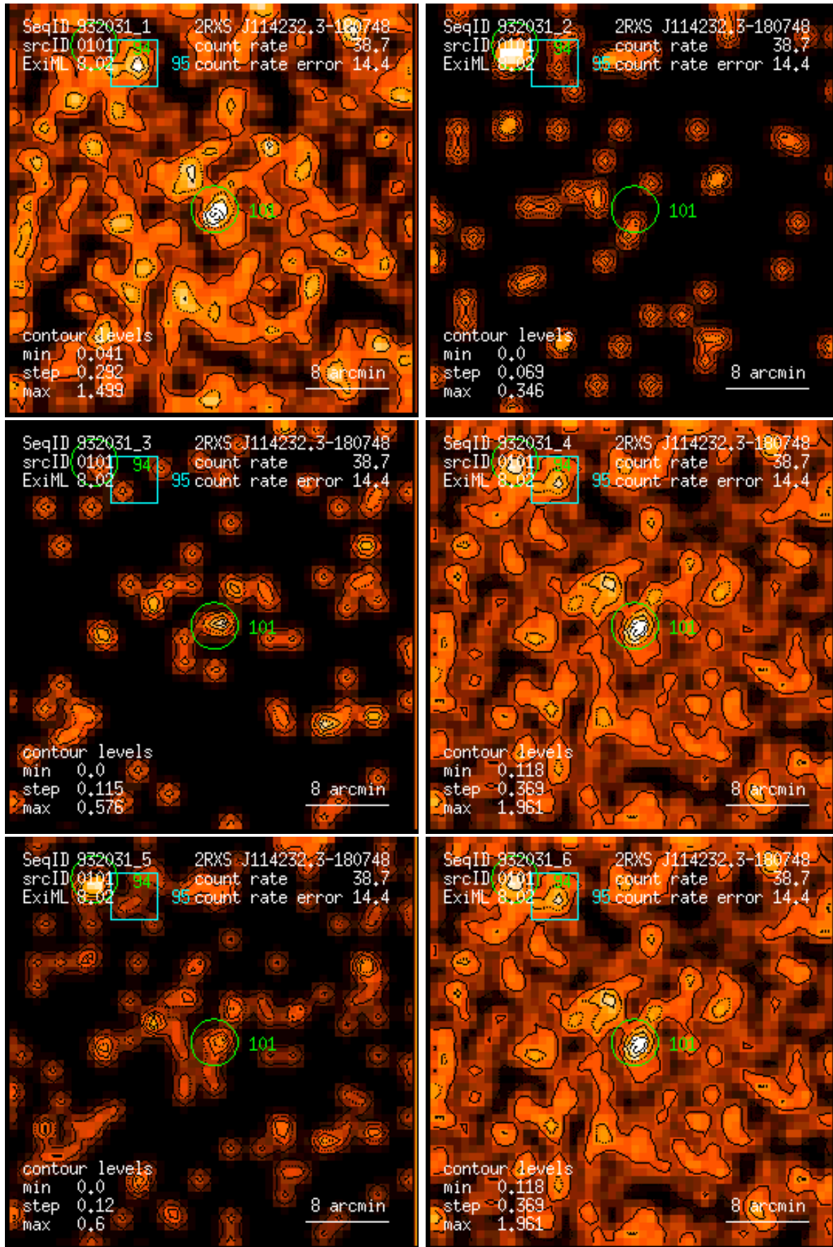
Figure 101: RASS 932031: detection 0101: band rate images, Gaussian filter: (1) PSPC channels 11 – 41, (2) 52 – 90, (3) 91 – 201, (4) 11 – 235, (5) 52 – 201, (6) 11 – 201. Broad band rates in counts/ks. Band rate contour levels in counts/ks/arcmin 2 .
