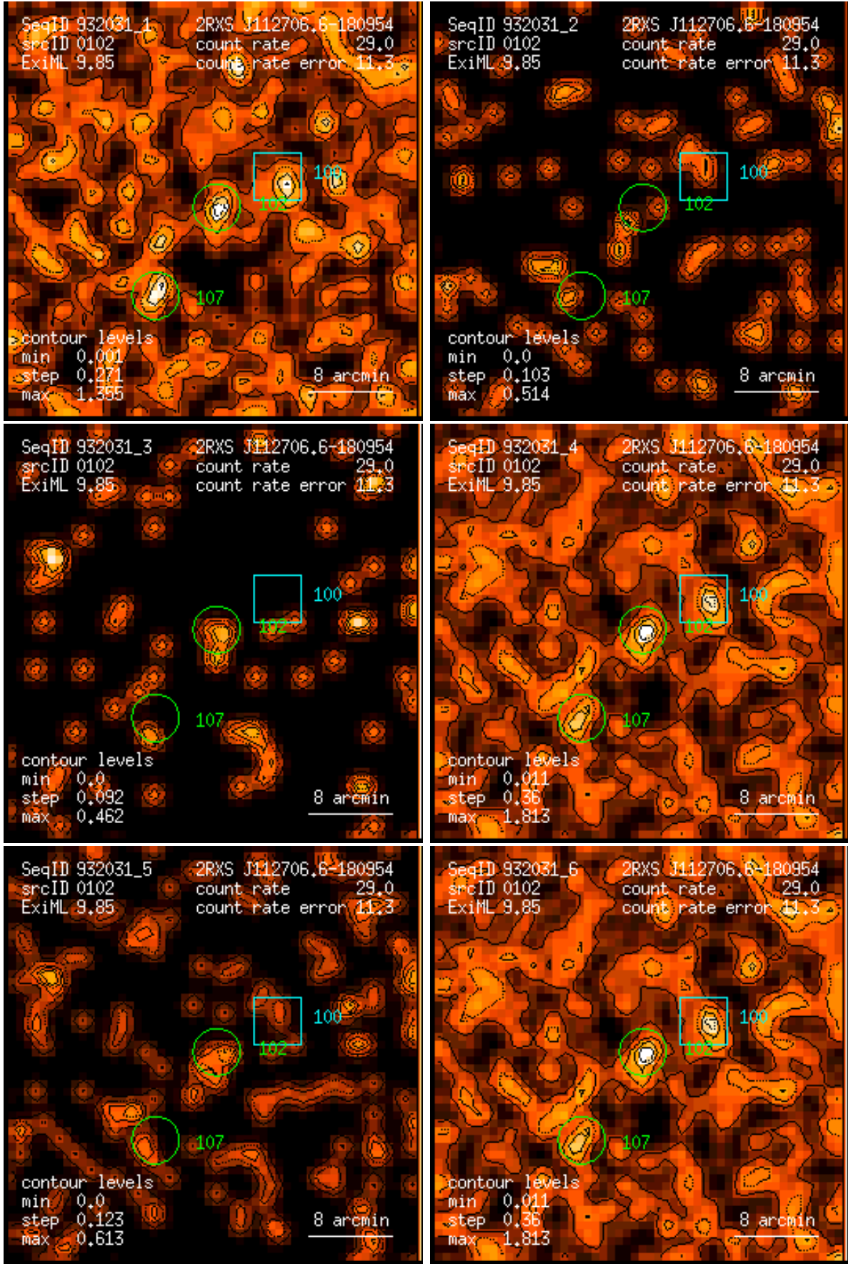
Figure 102: RASS 932031: detection 0102: band rate images, Gaussian filter: (1) PSPC channels 11 – 41, (2) 52 – 90, (3) 91 – 201, (4) 11 – 235, (5) 52 – 201, (6) 11 – 201. Broad band rates in counts/ks. Band rate contour levels in counts/ks/arcmin 2 .
