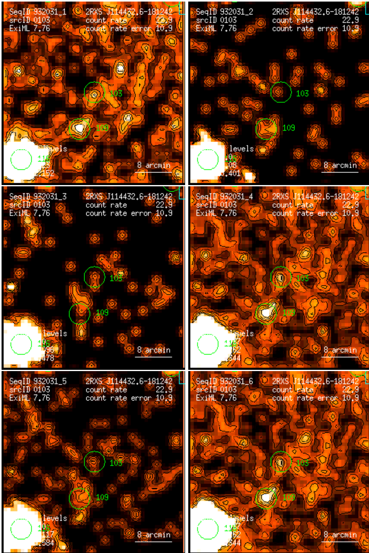
Figure 103: RASS 932031: detection 0103: band rate images, Gaussian filter: (1) PSPC channels 11 – 41, (2) 52 – 90, (3) 91 – 201, (4) 11 – 235, (5) 52 – 201, (6) 11 – 201. Broad band rates in counts/ks. Band rate contour levels in counts/ks/arcmin 2 .
