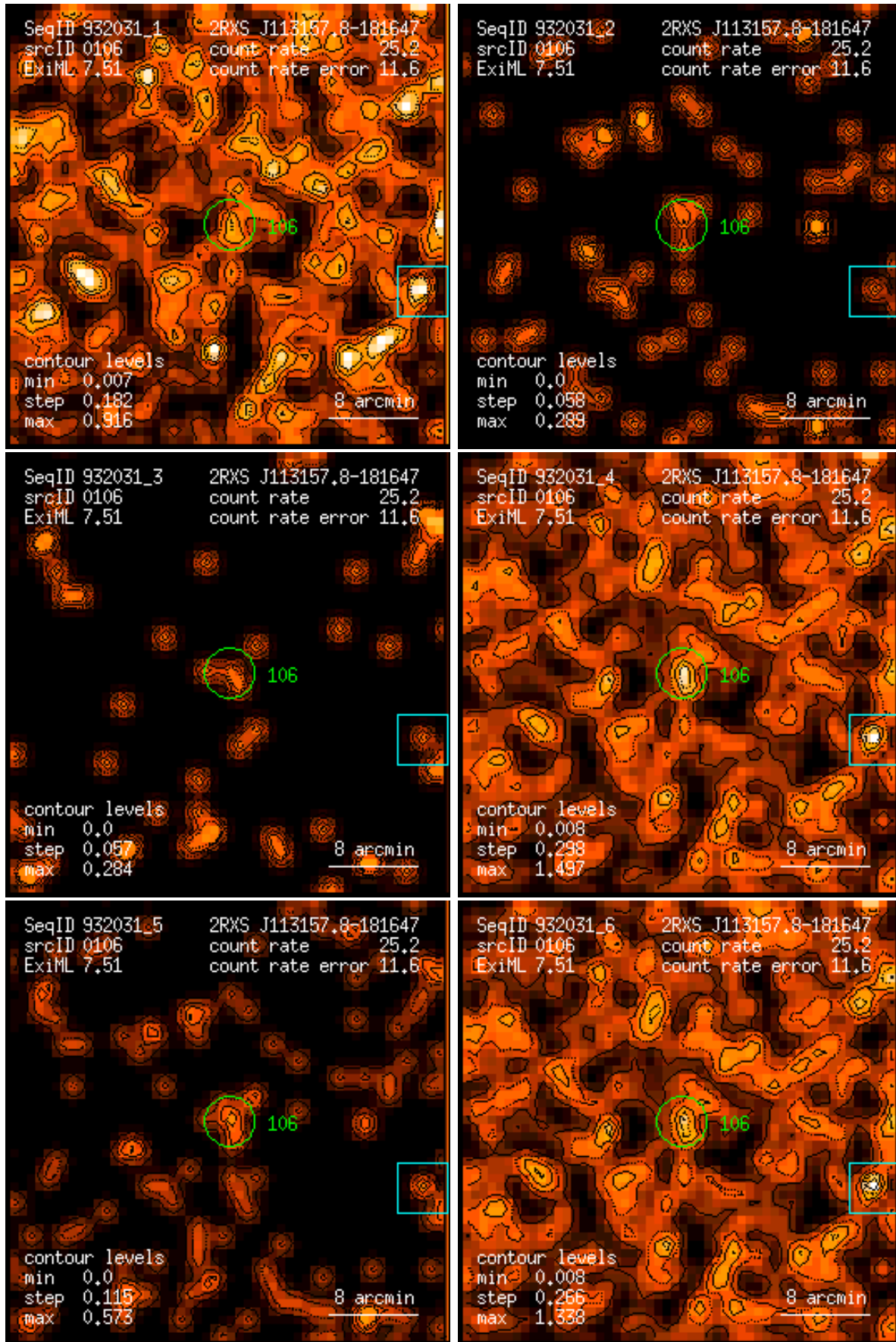
Figure 106: RASS 932031: detection 0106: band rate images, Gaussian filter: (1) PSPC channels 11 – 41, (2) 52 – 90, (3) 91 – 201, (4) 11 – 235, (5) 52 – 201, (6) 11 – 201. Broad band rates in counts/ks. Band rate contour levels in counts/ks/arcmin 2 .
