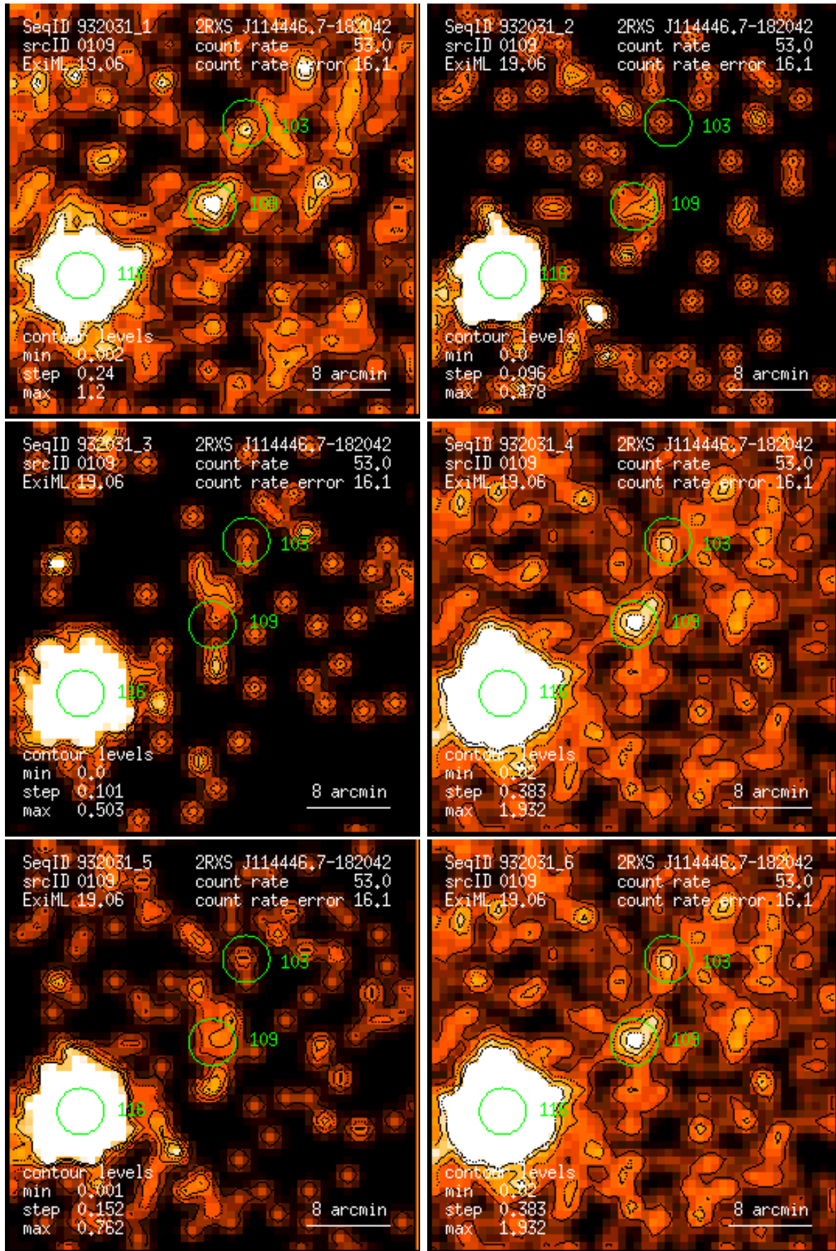
Figure 109: RASS 932031: detection 0109: band rate images, Gaussian filter: (1) PSPC channels 11 – 41, (2) 52 – 90, (3) 91 – 201, (4) 11 – 235, (5) 52 – 201, (6) 11 – 201. Broad band rates in counts/ks. Band rate contour levels in counts/ks/arcmin 2 .
