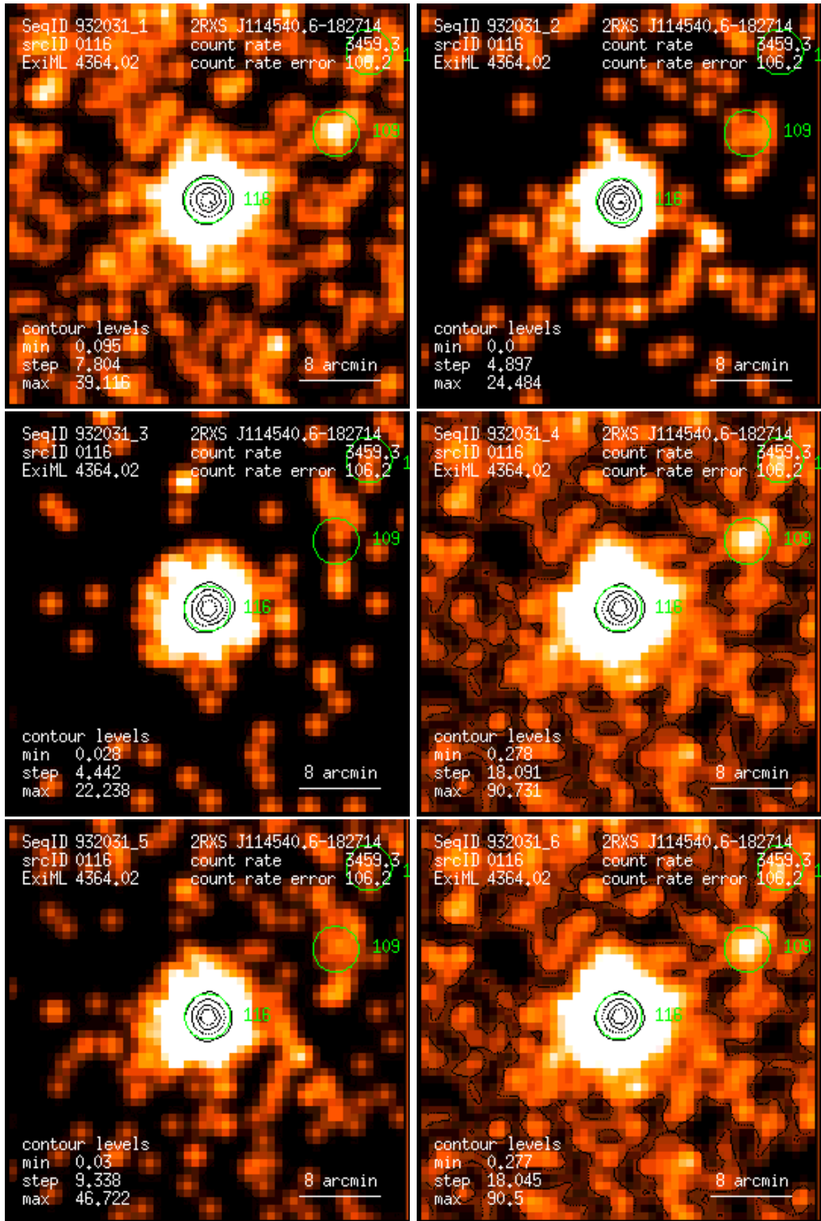
Figure 116: RASS 932031: detection 0116: band rate images, Gaussian filter: (1) PSPC channels 11 – 41, (2) 52 – 90, (3) 91 – 201, (4) 11 – 235, (5) 52 – 201, (6) 11 – 201. Broad band rates in counts/ks. Band rate contour levels in counts/ks/arcmin 2 .
