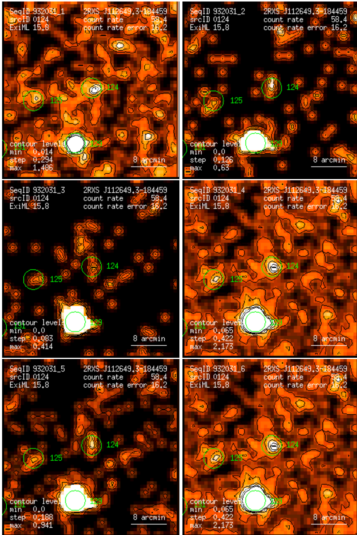
Figure 124: RASS 932031: detection 0124: band rate images, Gaussian filter: (1) PSPC channels 11 – 41, (2) 52 – 90, (3) 91 – 201, (4) 11 – 235, (5) 52 – 201, (6) 11 – 201. Broad band rates in counts/ks. Band rate contour levels in counts/ks/arcmin 2 .
