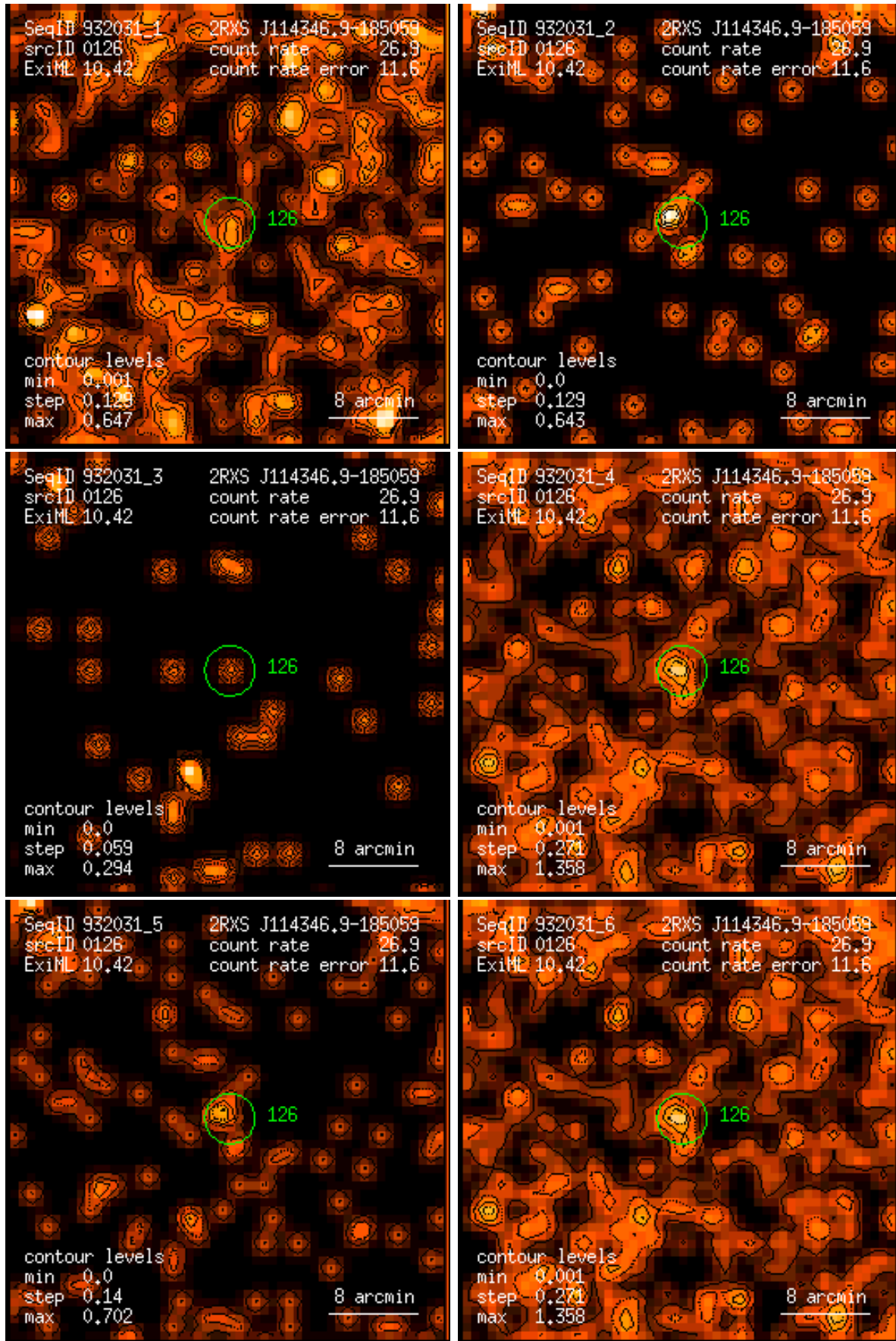
Figure 126: RASS 932031: detection 0126: band rate images, Gaussian filter: (1) PSPC channels 11 – 41, (2) 52 – 90, (3) 91 – 201, (4) 11 – 235, (5) 52 – 201, (6) 11 – 201. Broad band rates in counts/ks. Band rate contour levels in counts/ks/arcmin 2 .
