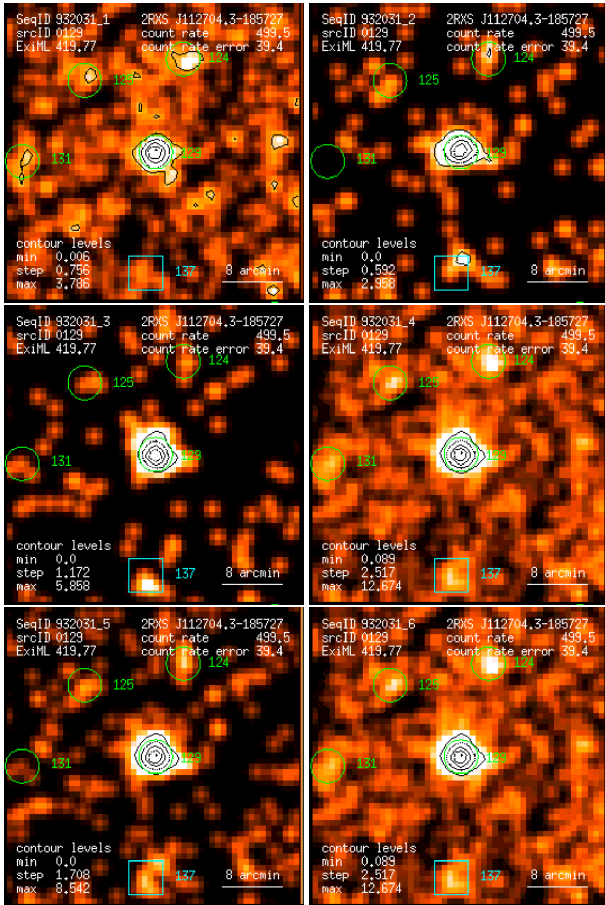
Figure 129: RASS 932031: detection 0129: band rate images, Gaussian filter: (1) PSPC channels 11 – 41, (2) 52 – 90, (3) 91 – 201, (4) 11 – 235, (5) 52 – 201, (6) 11 – 201. Broad band rates in counts/ks. Band rate contour levels in counts/ks/arcmin 2 .
