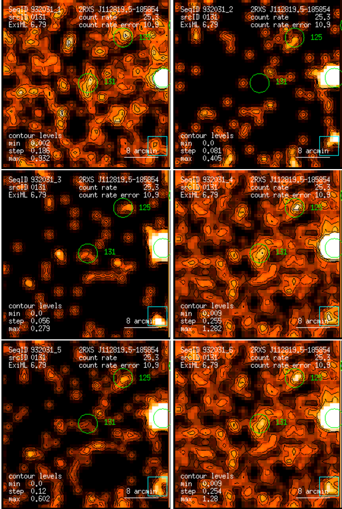
Figure 131: RASS 932031: detection 0131: band rate images, Gaussian filter: (1) PSPC channels 11 – 41, (2) 52 – 90, (3) 91 – 201, (4) 11 – 235, (5) 52 – 201, (6) 11 – 201. Broad band rates in counts/ks. Band rate contour levels in counts/ks/arcmin 2 .
