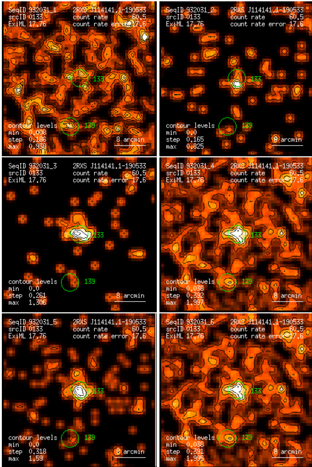
Figure 133: RASS 932031: detection 0133: band rate images, Gaussian filter: (1) PSPC channels 11 – 41, (2) 52 – 90, (3) 91 – 201, (4) 11 – 235, (5) 52 – 201, (6) 11 – 201. Broad band rates in counts/ks. Band rate contour levels in counts/ks/arcmin 2 .
