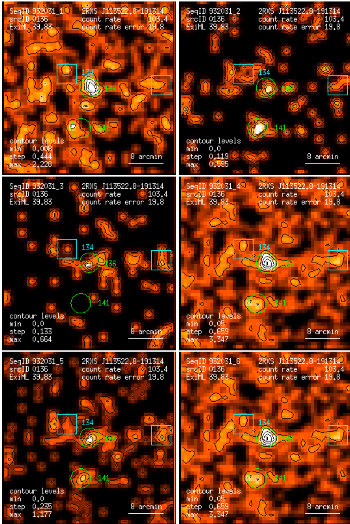
Figure 136: RASS 932031: detection 0136: band rate images, Gaussian filter: (1) PSPC channels 11 – 41, (2) 52 – 90, (3) 91 – 201, (4) 11 – 235, (5) 52 – 201, (6) 11 – 201. Broad band rates in counts/ks. Band rate contour levels in counts/ks/arcmin 2 .
