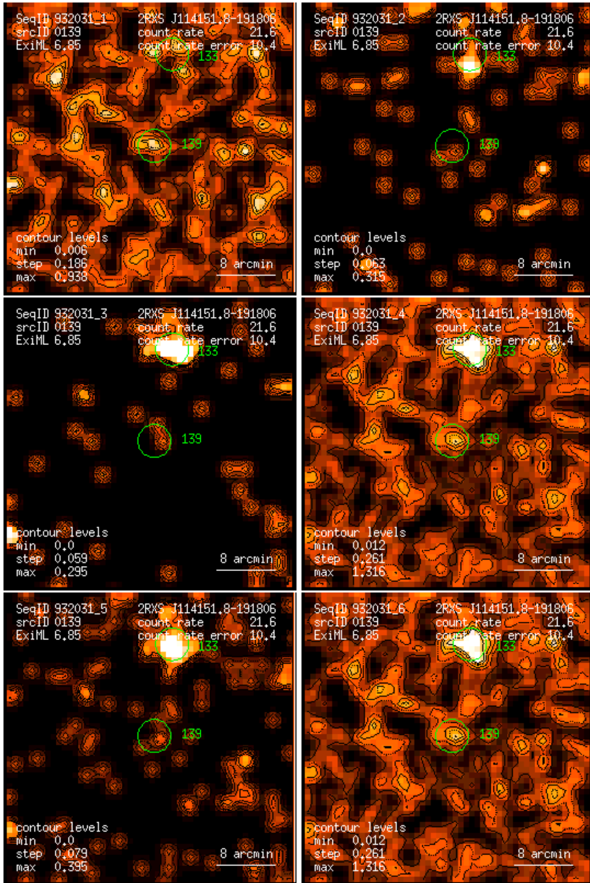
Figure 139: RASS 932031: detection 0139: band rate images, Gaussian filter: (1) PSPC channels 11 – 41, (2) 52 – 90, (3) 91 – 201, (4) 11 – 235, (5) 52 – 201, (6) 11 – 201. Broad band rates in counts/ks. Band rate contour levels in counts/ks/arcmin 2 .
