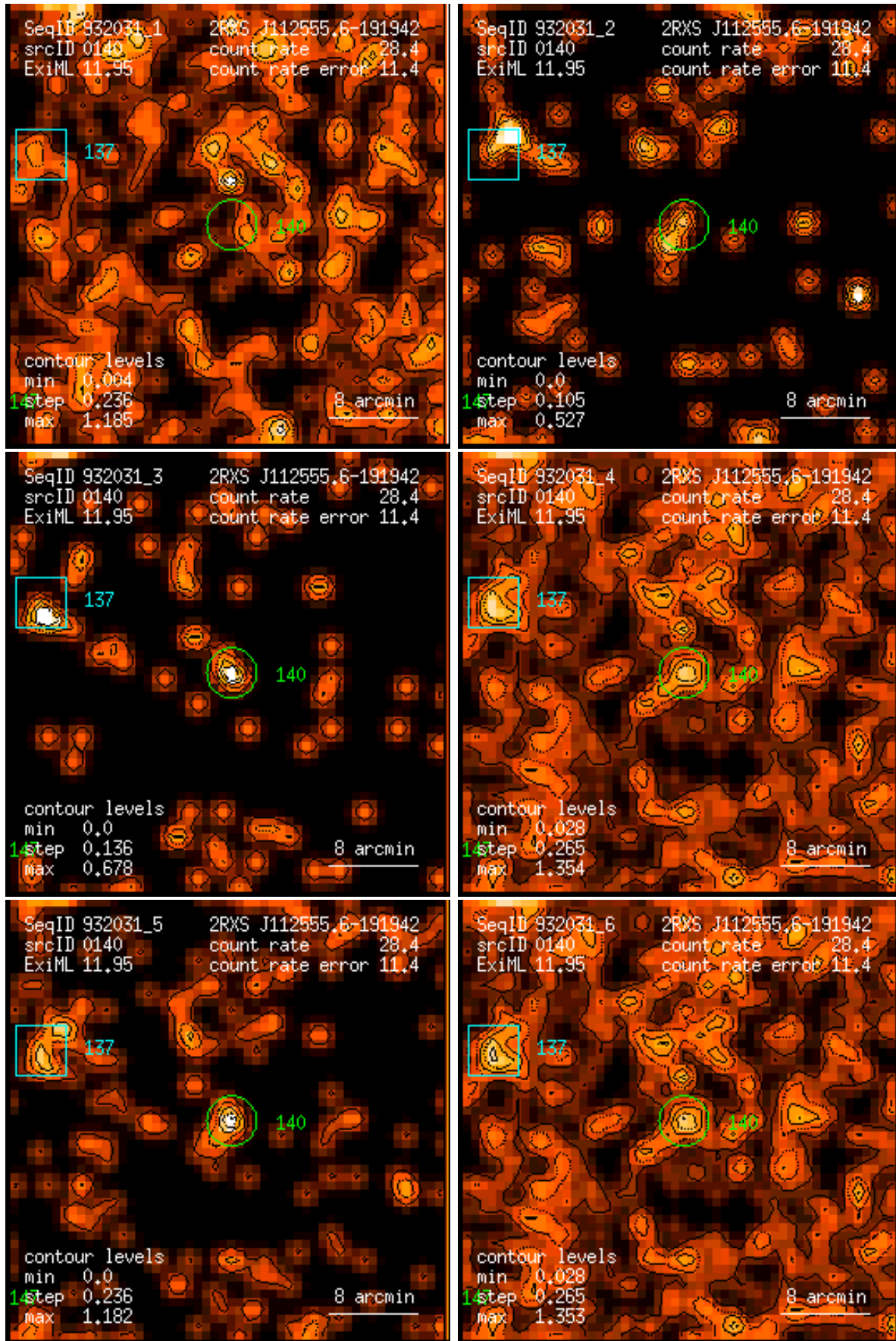
Figure 140: RASS 932031: detection 0140: band rate images, Gaussian filter: (1) PSPC channels 11 – 41, (2) 52 – 90, (3) 91 – 201, (4) 11 – 235, (5) 52 – 201, (6) 11 – 201. Broad band rates in counts/ks. Band rate contour levels in counts/ks/arcmin 2 .
