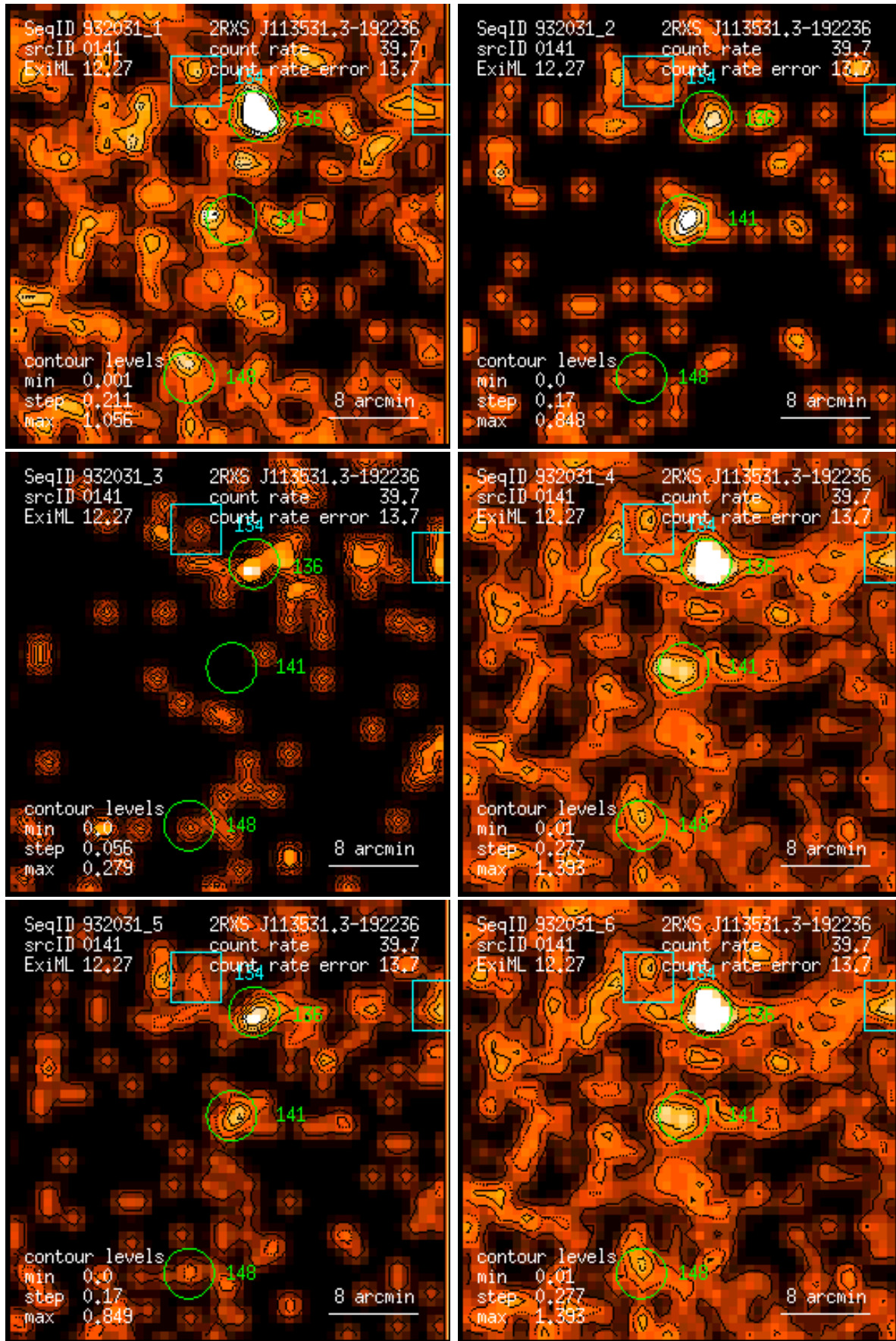
Figure 141: RASS 932031: detection 0141: band rate images, Gaussian filter: (1) PSPC channels 11 – 41, (2) 52 – 90, (3) 91 – 201, (4) 11 – 235, (5) 52 – 201, (6) 11 – 201. Broad band rates in counts/ks. Band rate contour levels in counts/ks/arcmin 2 .
