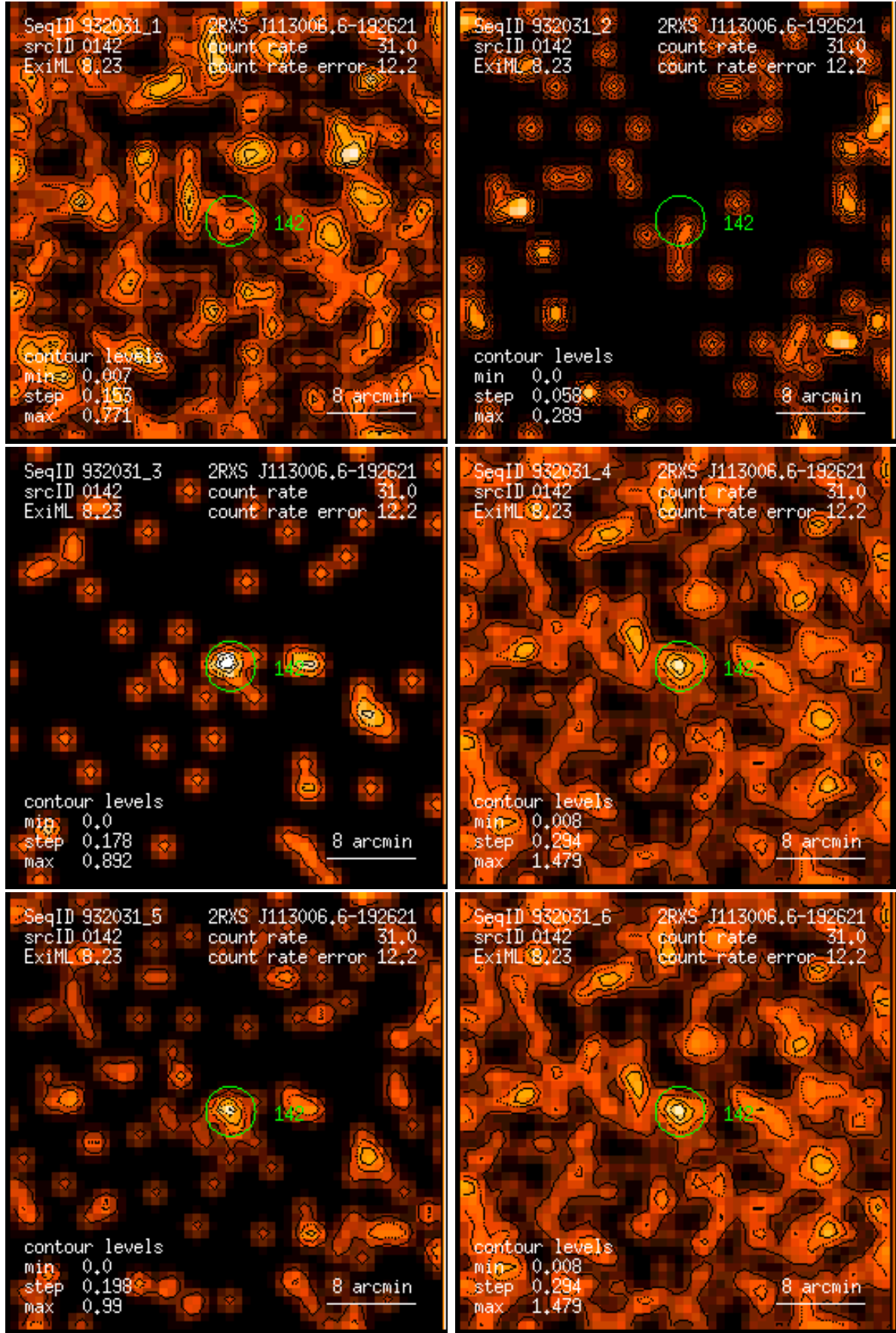
Figure 142: RASS 932031: detection 0142: band rate images, Gaussian filter: (1) PSPC channels 11 – 41, (2) 52 – 90, (3) 91 – 201, (4) 11 – 235, (5) 52 – 201, (6) 11 – 201. Broad band rates in counts/ks. Band rate contour levels in counts/ks/arcmin 2 .
