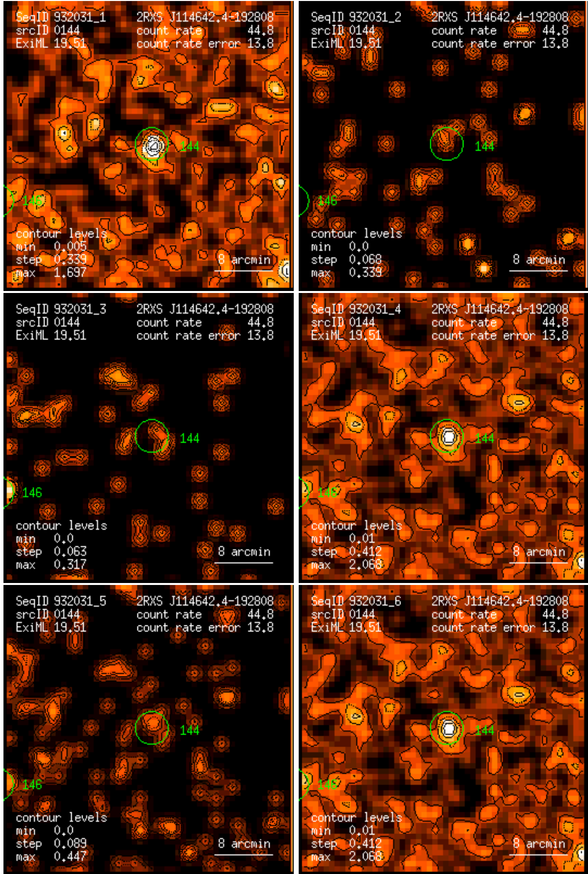
Figure 144: RASS 932031: detection 0144: band rate images, Gaussian filter: (1) PSPC channels 11 – 41, (2) 52 – 90, (3) 91 – 201, (4) 11 – 235, (5) 52 – 201, (6) 11 – 201. Broad band rates in counts/ks. Band rate contour levels in counts/ks/arcmin 2 .
