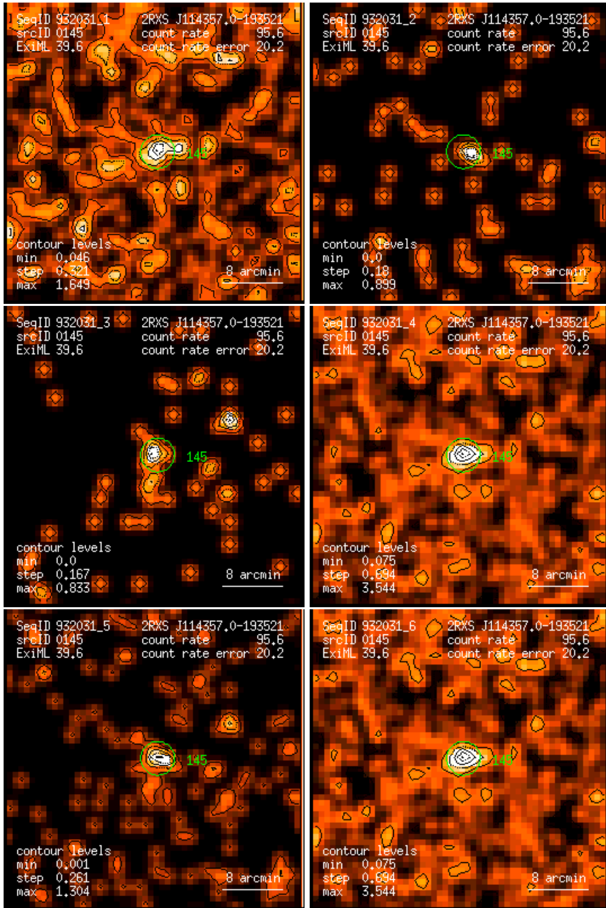
Figure 145: RASS 932031: detection 0145: band rate images, Gaussian filter: (1) PSPC channels 11 – 41, (2) 52 – 90, (3) 91 – 201, (4) 11 – 235, (5) 52 – 201, (6) 11 – 201. Broad band rates in counts/ks. Band rate contour levels in counts/ks/arcmin 2 .
