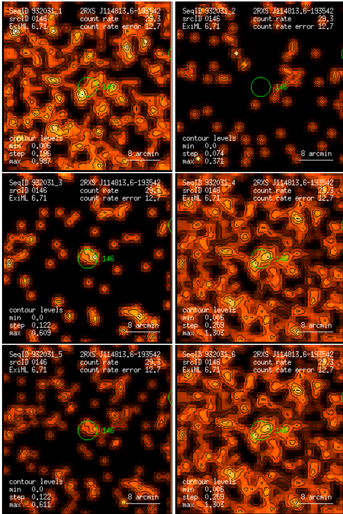
Figure 146: RASS 932031: detection 0146: band rate images, Gaussian filter: (1) PSPC channels 11 – 41, (2) 52 – 90, (3) 91 – 201, (4) 11 – 235, (5) 52 – 201, (6) 11 – 201. Broad band rates in counts/ks. Band rate contour levels in counts/ks/arcmin 2 .
