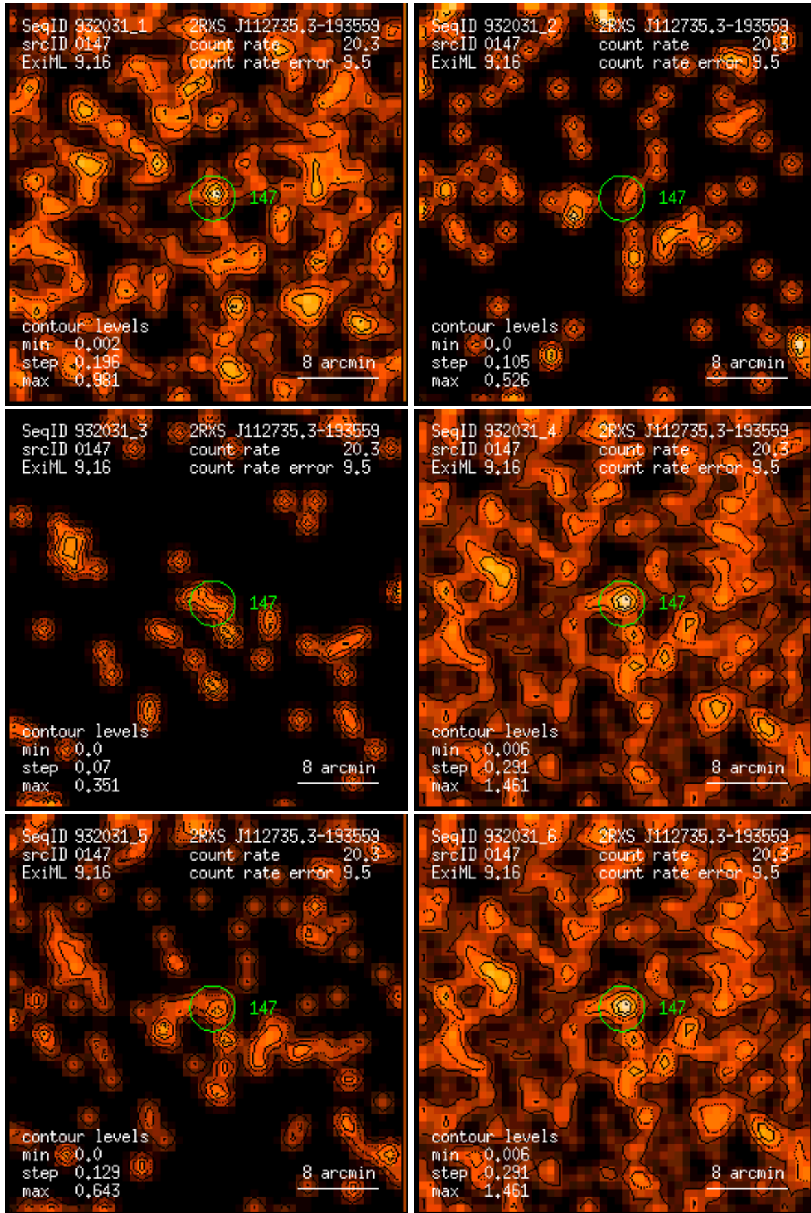
Figure 147: RASS 932031: detection 0147: band rate images, Gaussian filter: (1) PSPC channels 11 – 41, (2) 52 – 90, (3) 91 – 201, (4) 11 – 235, (5) 52 – 201, (6) 11 – 201. Broad band rates in counts/ks. Band rate contour levels in counts/ks/arcmin 2 .
