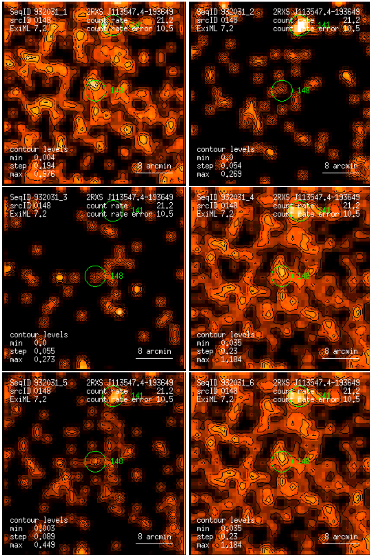
Figure 148: RASS 932031: detection 0148: band rate images, Gaussian filter: (1) PSPC channels 11 – 41, (2) 52 – 90, (3) 91 – 201, (4) 11 – 235, (5) 52 – 201, (6) 11 – 201. Broad band rates in counts/ks. Band rate contour levels in counts/ks/arcmin 2 .
