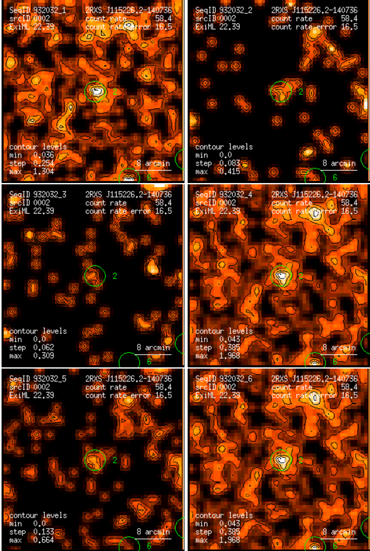
Figure 2: RASS 932032: detection 0002: band rate images, Gaussian filter: (1) PSPC channels 11 – 41, (2) 52 – 90, (3) 91 – 201, (4) 11 – 235, (5) 52 – 201, (6) 11 – 201. Broad band rates in counts/ks. Band rate contour levels in counts/ks/arcmin 2 .
