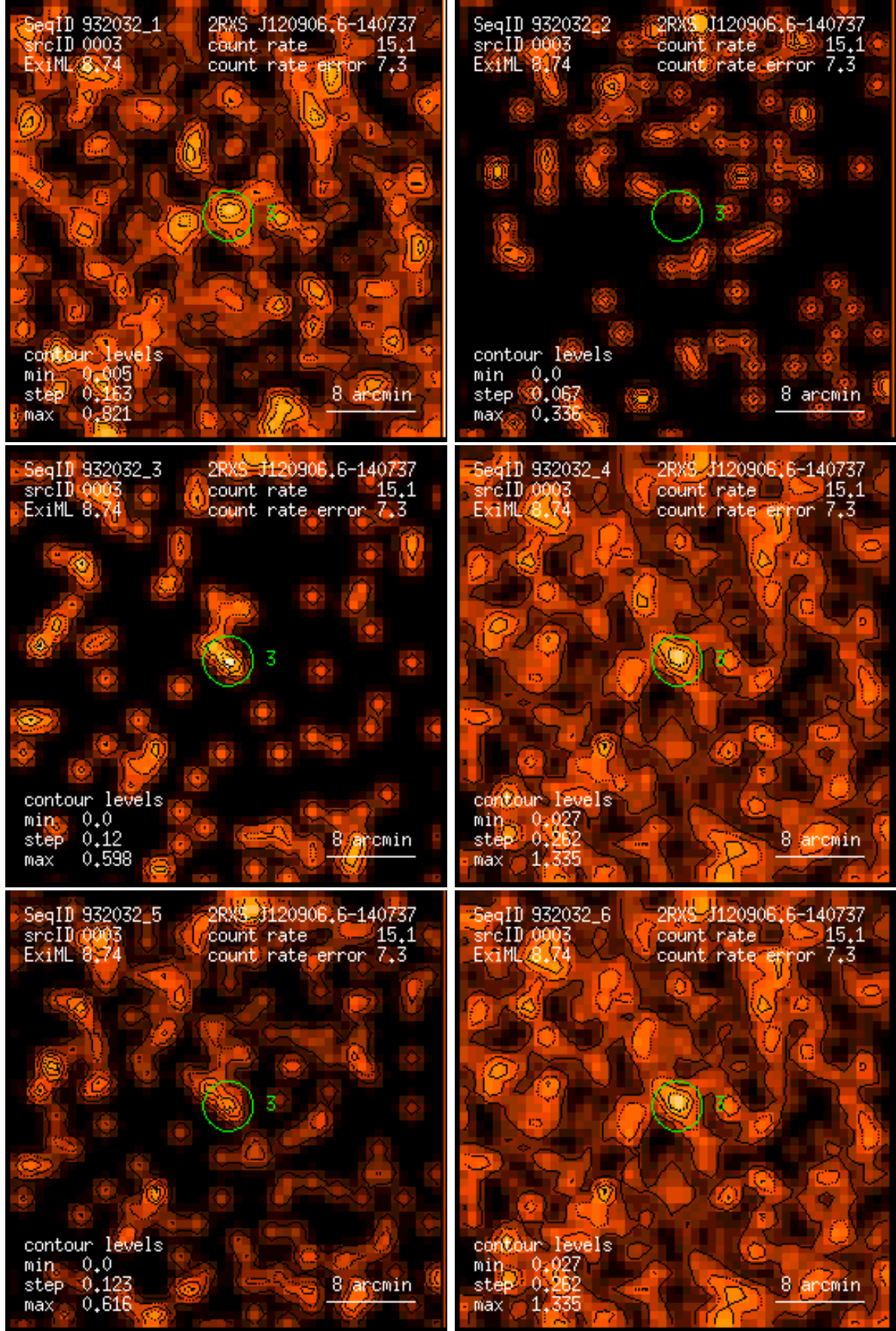
Figure 3: RASS 932032: detection 0003: band rate images, Gaussian filter: (1) PSPC channels 11 – 41, (2) 52 – 90, (3) 91 – 201, (4) 11 – 235, (5) 52 – 201, (6) 11 – 201. Broad band rates in counts/ks. Band rate contour levels in counts/ks/arcmin 2 .
