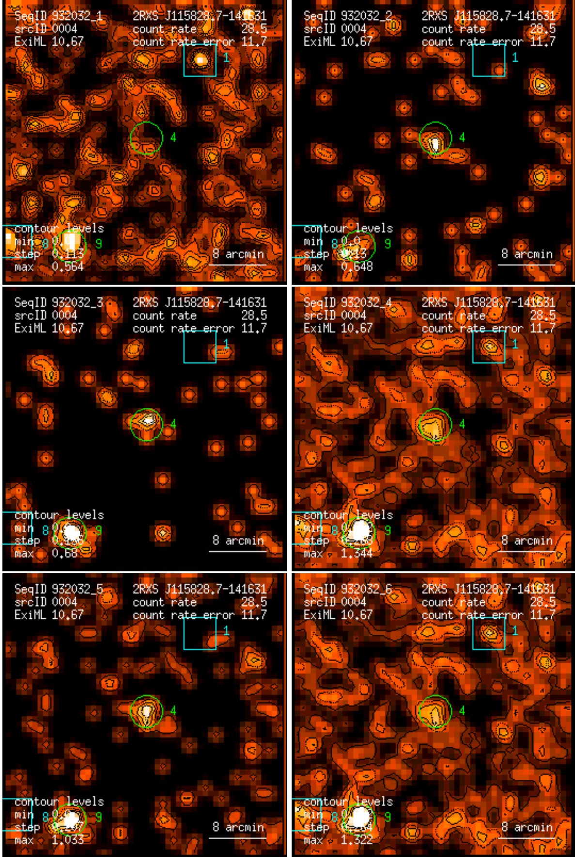
Figure 4: RASS 932032: detection 0004: band rate images, Gaussian filter: (1) PSPC channels 11 – 41, (2) 52 – 90, (3) 91 – 201, (4) 11 – 235, (5) 52 – 201, (6) 11 – 201. Broad band rates in counts/ks. Band rate contour levels in counts/ks/arcmin 2 .
