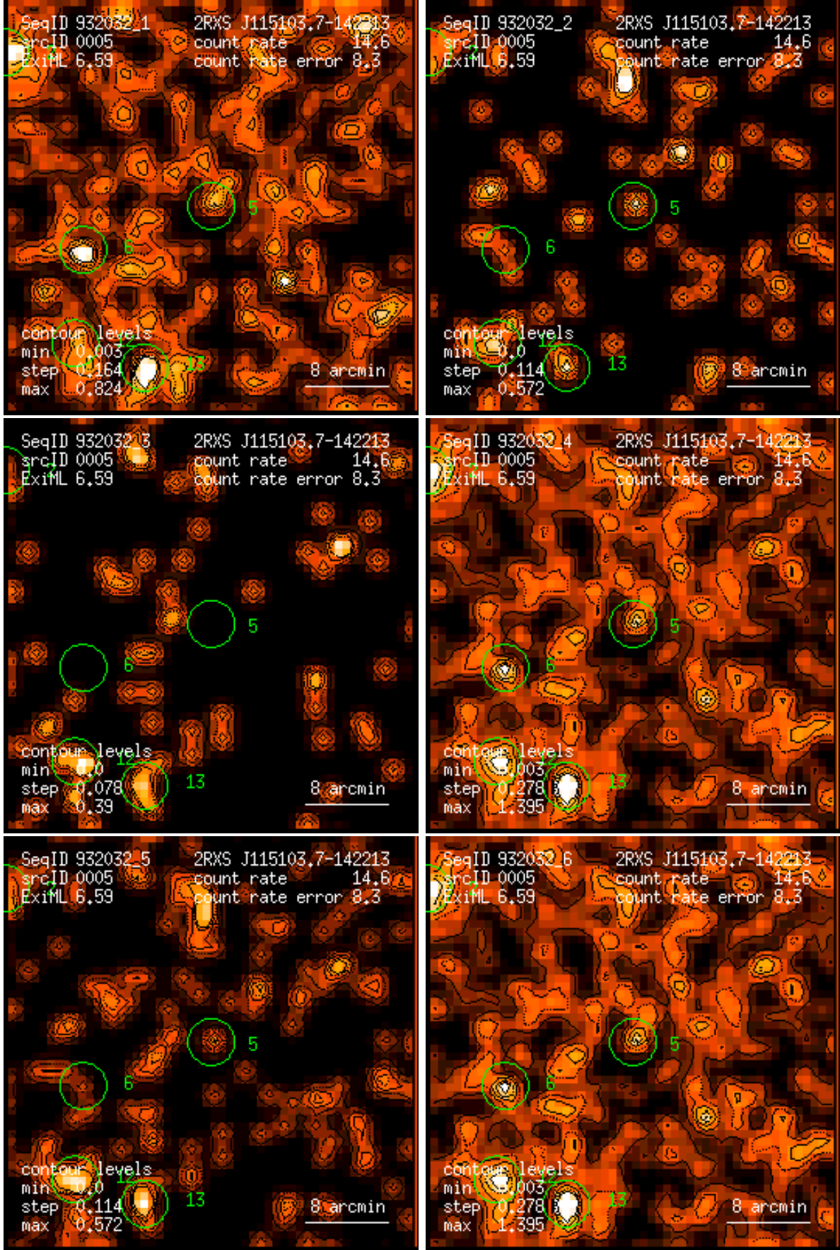
Figure 5: RASS 932032: detection 0005: band rate images, Gaussian filter: (1) PSPC channels 11 – 41, (2) 52 – 90, (3) 91 – 201, (4) 11 – 235, (5) 52 – 201, (6) 11 – 201. Broad band rates in counts/ks. Band rate contour levels in counts/ks/arcmin 2 .
