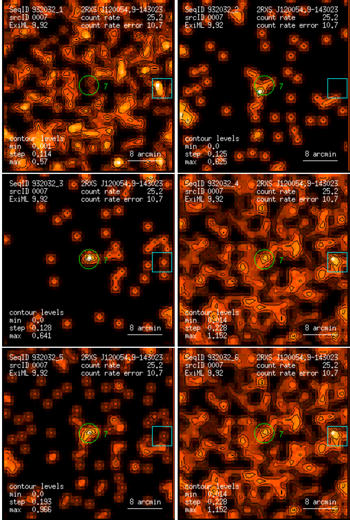
Figure 7: RASS 932032: detection 0007: band rate images, Gaussian filter: (1) PSPC channels 11 – 41, (2) 52 – 90, (3) 91 – 201, (4) 11 – 235, (5) 52 – 201, (6) 11 – 201. Broad band rates in counts/ks. Band rate contour levels in counts/ks/arcmin 2 .
