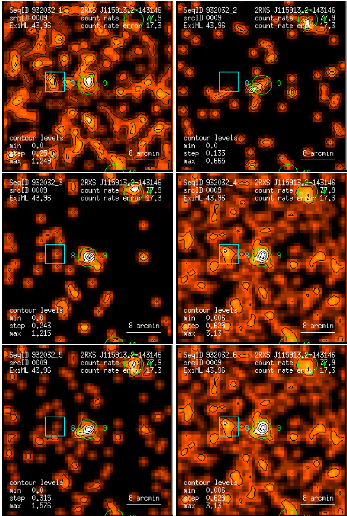
Figure 9: RASS 932032: detection 0009: band rate images, Gaussian filter: (1) PSPC channels 11 – 41, (2) 52 – 90, (3) 91 – 201, (4) 11 – 235, (5) 52 – 201, (6) 11 – 201. Broad band rates in counts/ks. Band rate contour levels in counts/ks/arcmin 2 .
