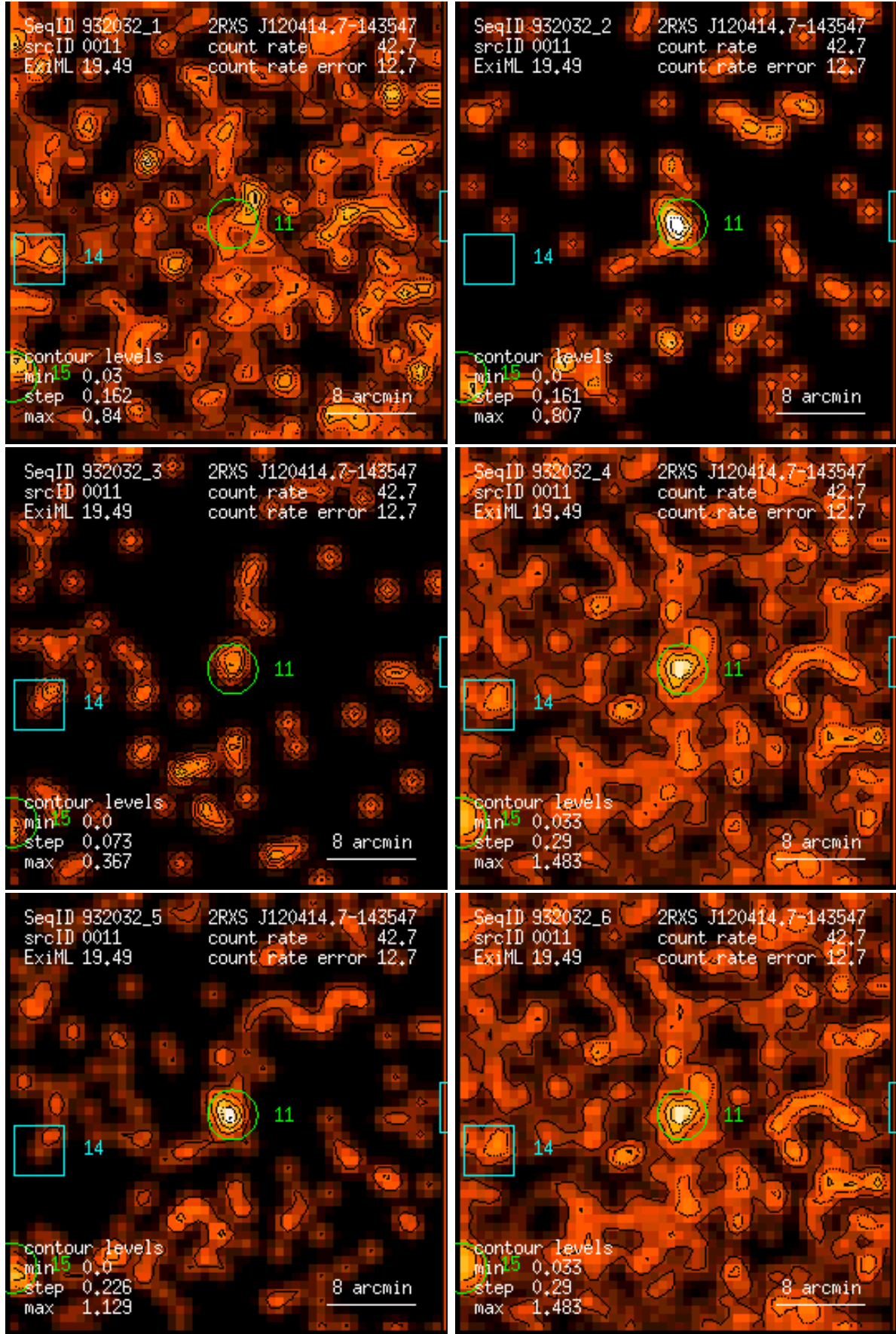
Figure 11: RASS 932032: detection 0011: band rate images, Gaussian filter: (1) PSPC channels 11 – 41, (2) 52 – 90, (3) 91 – 201, (4) 11 – 235, (5) 52 – 201, (6) 11 – 201. Broad band rates in counts/ks. Band rate contour levels in counts/ks/arcmin 2 .
