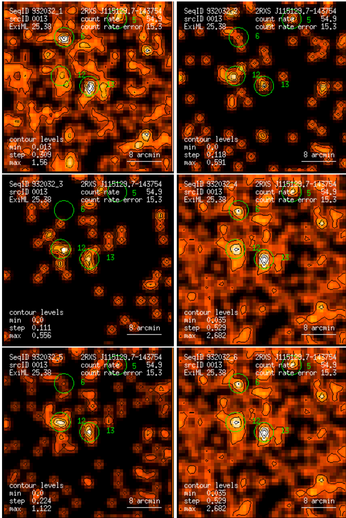
Figure 13: RASS 932032: detection 0013: band rate images, Gaussian filter: (1) PSPC channels 11 – 41, (2) 52 – 90, (3) 91 – 201, (4) 11 – 235, (5) 52 – 201, (6) 11 – 201. Broad band rates in counts/ks. Band rate contour levels in counts/ks/arcmin 2 .
