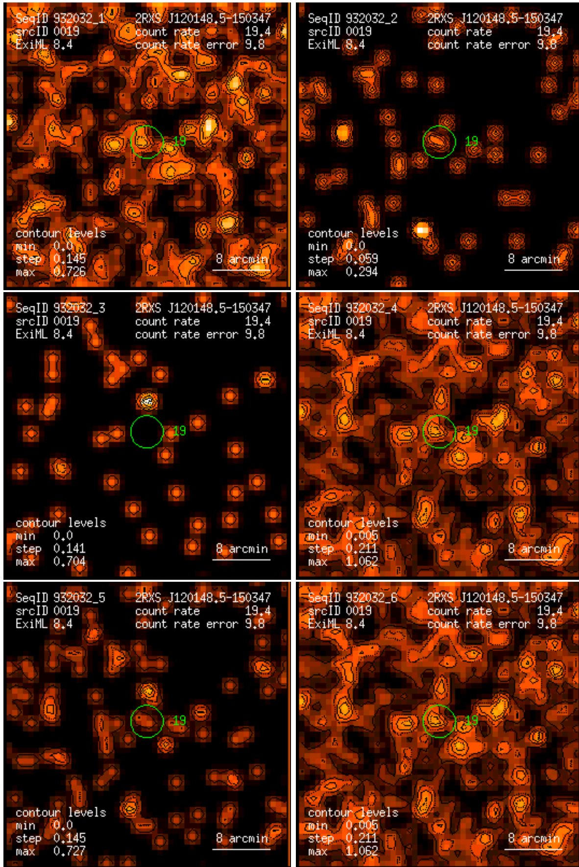
Figure 19: RASS 932032: detection 0019: band rate images, Gaussian filter: (1) PSPC channels 11 – 41, (2) 52 – 90, (3) 91 – 201, (4) 11 – 235, (5) 52 – 201, (6) 11 – 201. Broad band rates in counts/ks. Band rate contour levels in counts/ks/arcmin 2 .
