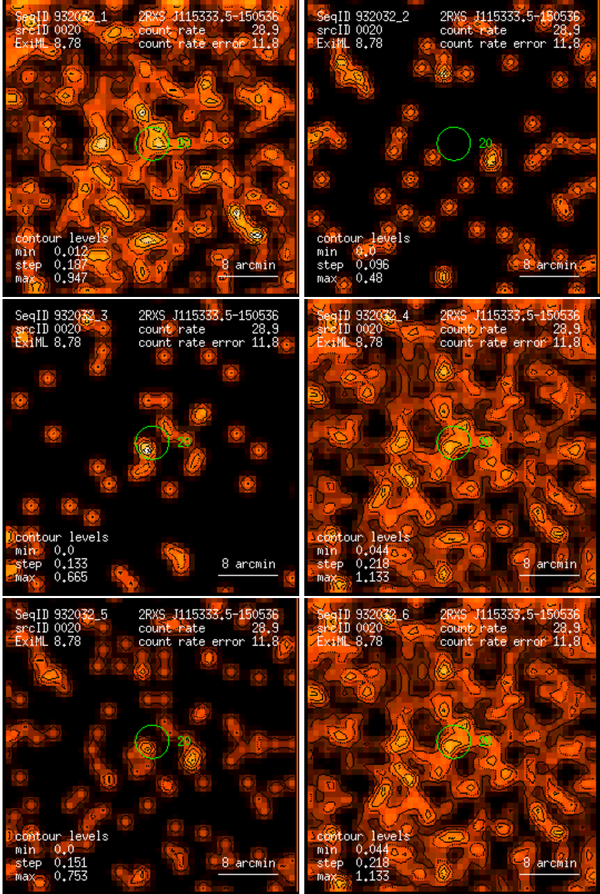
Figure 20: RASS 932032: detection 0020: band rate images, Gaussian filter: (1) PSPC channels 11 – 41, (2) 52 – 90, (3) 91 – 201, (4) 11 – 235, (5) 52 – 201, (6) 11 – 201. Broad band rates in counts/ks. Band rate contour levels in counts/ks/arcmin 2 .
