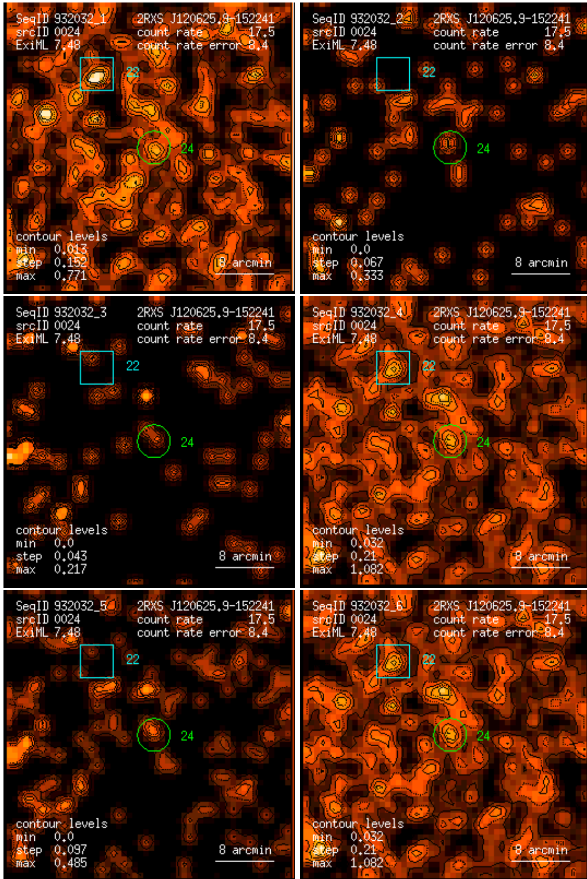
Figure 24: RASS 932032: detection 0024: band rate images, Gaussian filter: (1) PSPC channels 11 – 41, (2) 52 – 90, (3) 91 – 201, (4) 11 – 235, (5) 52 – 201, (6) 11 – 201. Broad band rates in counts/ks. Band rate contour levels in counts/ks/arcmin 2 .
