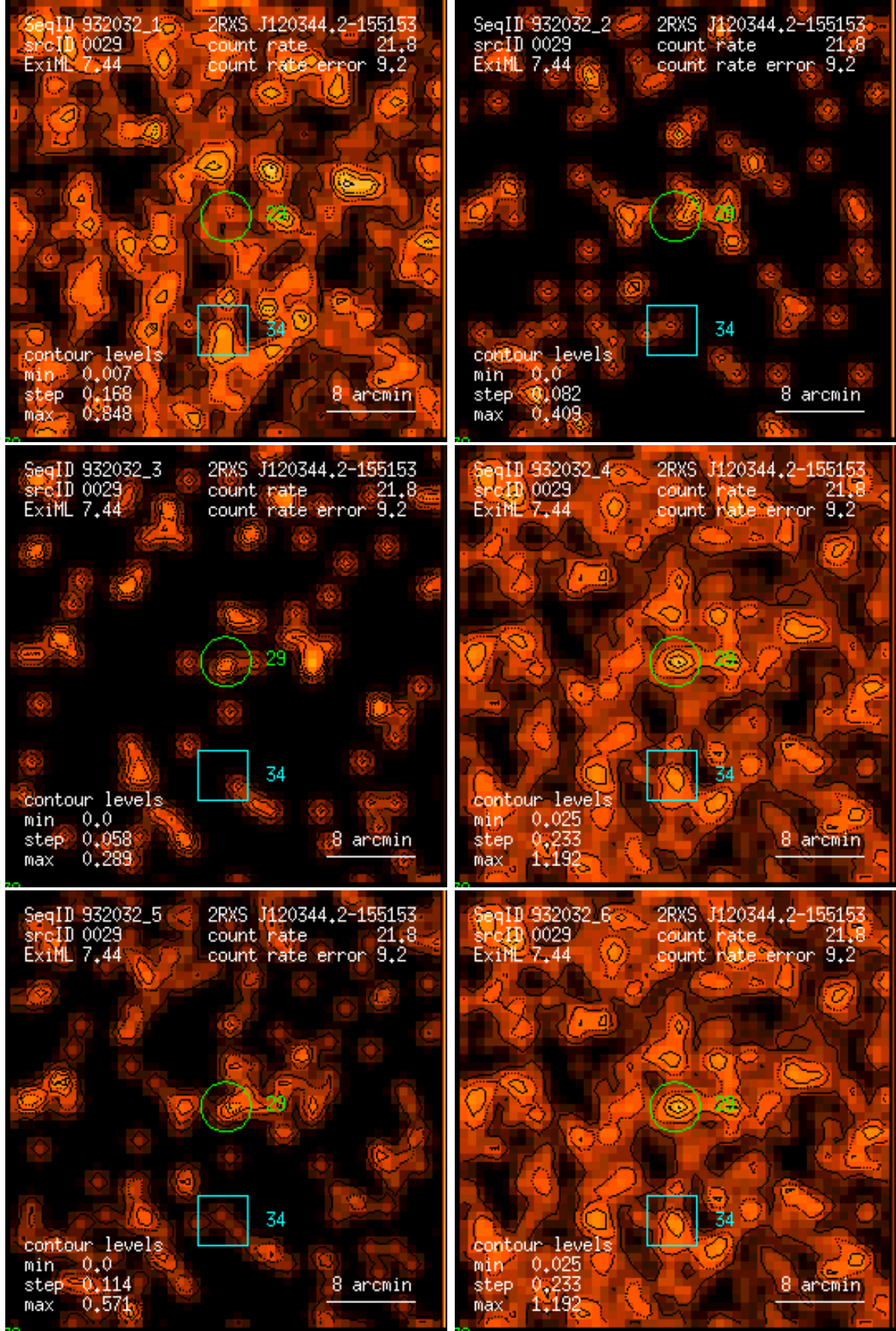
Figure 29: RASS 932032: detection 0029: band rate images, Gaussian filter: (1) PSPC channels 11 – 41, (2) 52 – 90, (3) 91 – 201, (4) 11 – 235, (5) 52 – 201, (6) 11 – 201. Broad band rates in counts/ks. Band rate contour levels in counts/ks/arcmin 2 .
