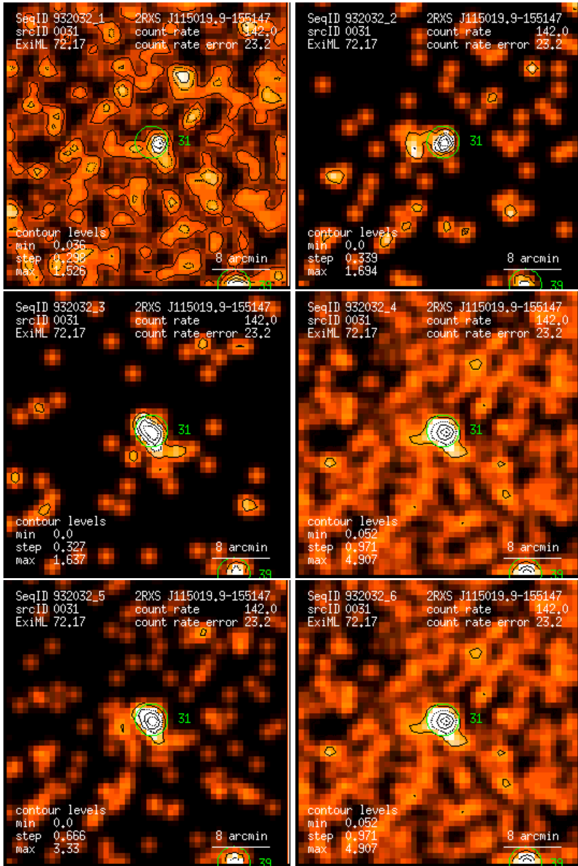
Figure 31: RASS 932032: detection 0031: band rate images, Gaussian filter: (1) PSPC channels 11 – 41, (2) 52 – 90, (3) 91 – 201, (4) 11 – 235, (5) 52 – 201, (6) 11 – 201. Broad band rates in counts/ks. Band rate contour levels in counts/ks/arcmin 2 .
